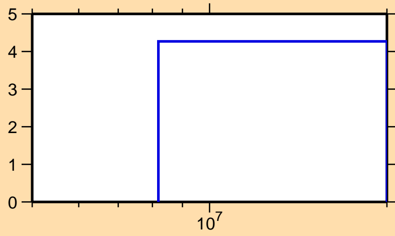
\Delta\sigma/\sigma vs. E for ^{164}\text{Hf}(n,\text{nonel.})
