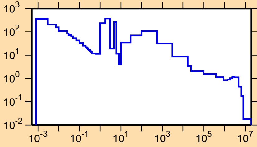
\sigma vs. E for ^{164}\text{Hf}(n,\gamma)
