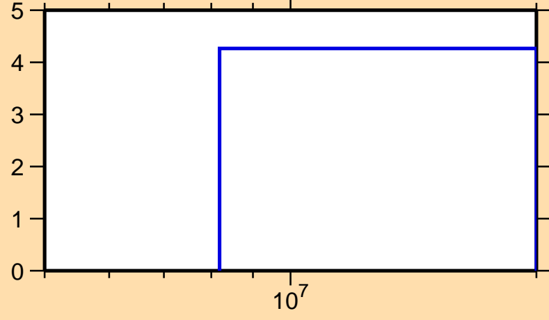
\Delta\sigma/\sigma vs. E for ^{164}\text{Hf}(n,\text{el.})
