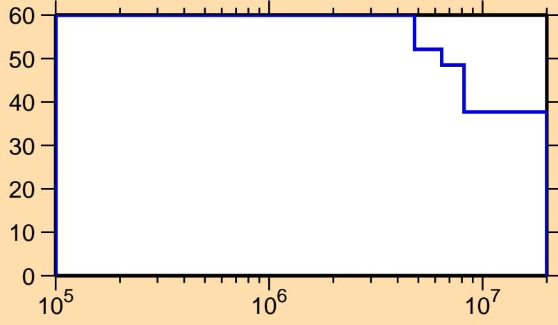
\Delta\sigma/\sigma vs. E for ^{164}\text{Hf}(n,n_1)
