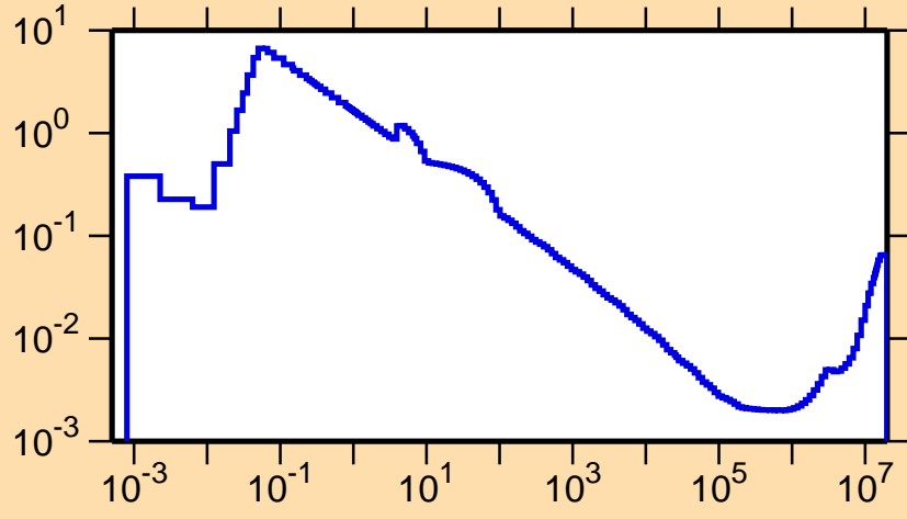
\sigma vs. E for ^{165}\text{Hf}(n,\alpha)
