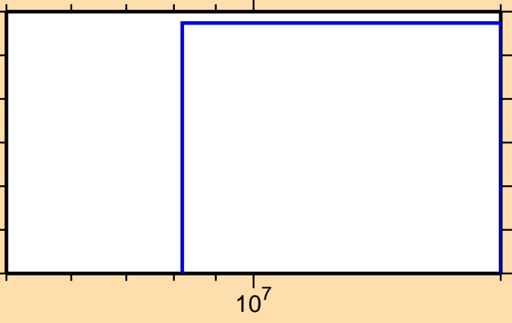
\sigma vs. E for ^{165}\text{Hf}(n,2n\alpha)
