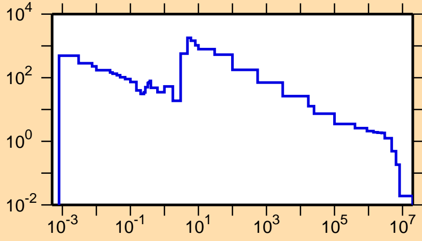
\sigma vs. E for ^{165}\text{Hf}(n,\gamma)
