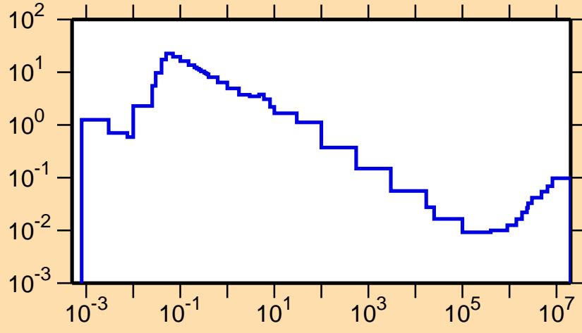
\sigma vs. E for ^{165}\text{Hf}(n,p)
