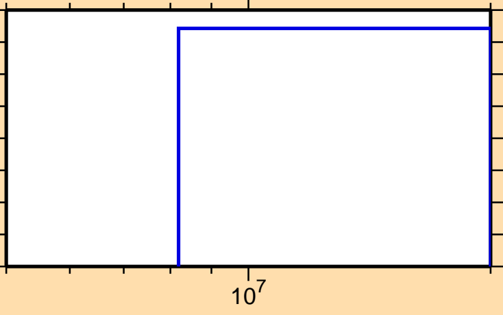
\sigma vs. E for ^{165}\text{Hf}(n,\text{pd})
