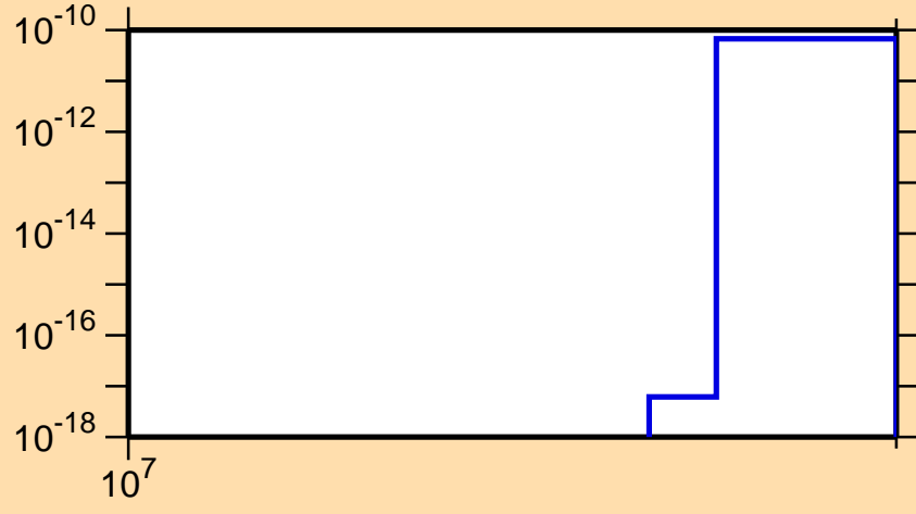
\sigma vs. E for ^{166}\text{Hf}(n,nt)
