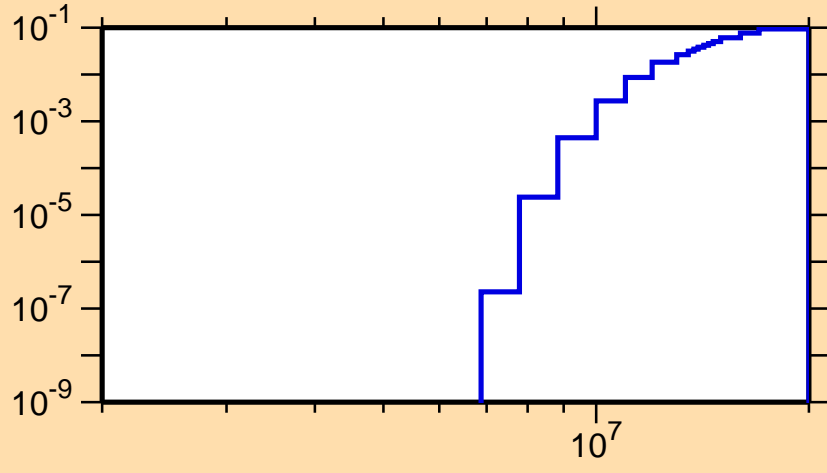
\sigma vs. E for ^{166}\text{Hf}(n,np)
