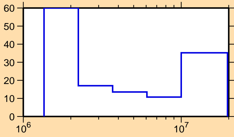
\Delta\sigma/\sigma vs. E for ^{166}\text{Hf}(n,n\text{cont.})
