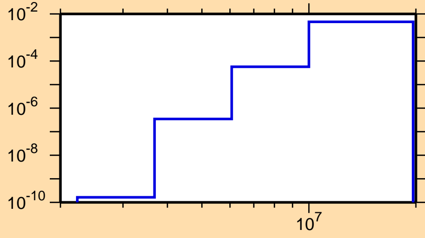
\sigma vs. E for ^{166}\text{Hf}(n,n\alpha)
