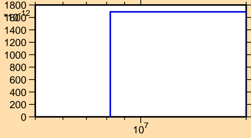
\sigma vs. E for ^{166}\text{Hf} (mt 45)
