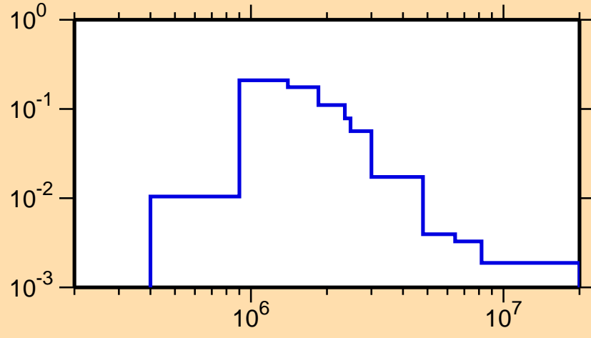
\sigma vs. E for ^{166}\text{Hf}(n,n_3)
