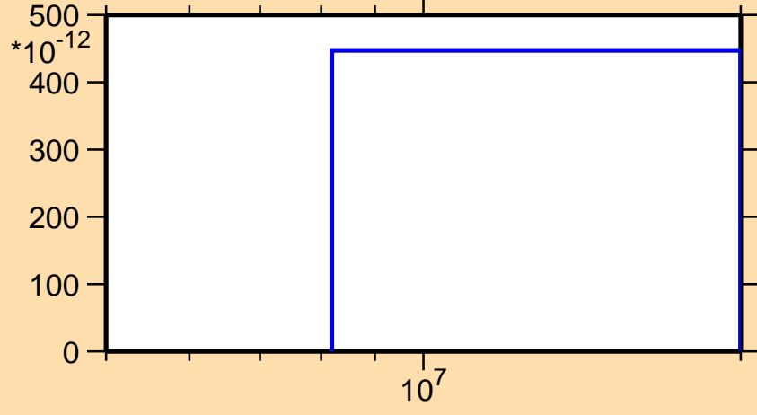
\sigma vs. E for ^{166}\text{Hf}(n,nd)
