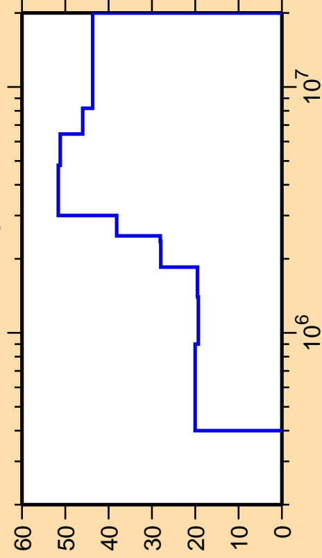
\Delta\sigma/\sigma vs. E for ^{166}\text{Hf}(n,n_3)
