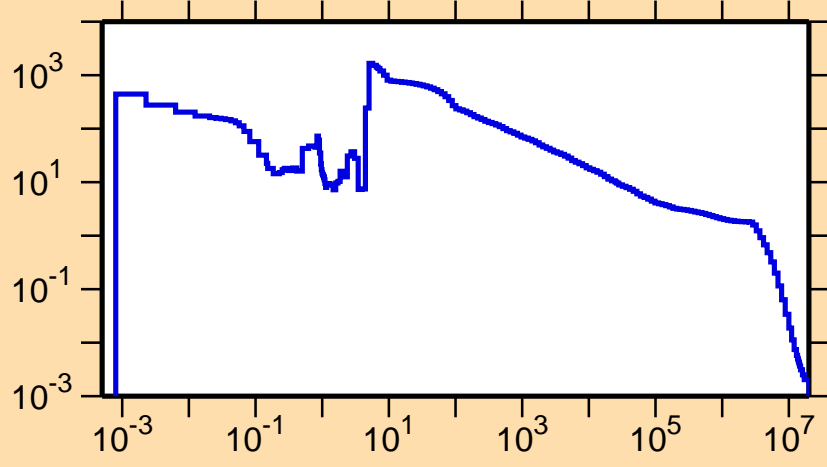
\sigma vs. E for ^{167}\text{Hf}(n,\gamma)
