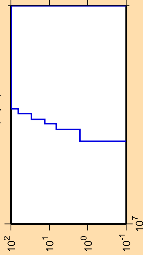
\Delta\sigma/\sigma vs. E for ^{167}\text{Hf}(n,pd)
