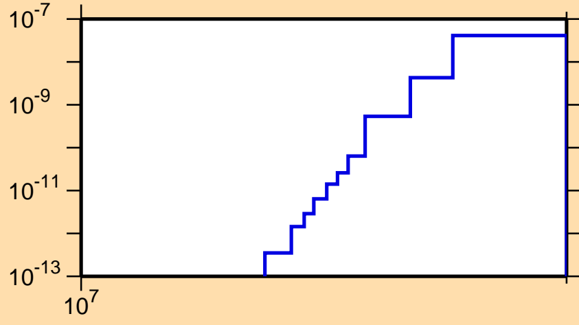
\sigma vs. E for ^{167}\text{Hf}(n,pd)
