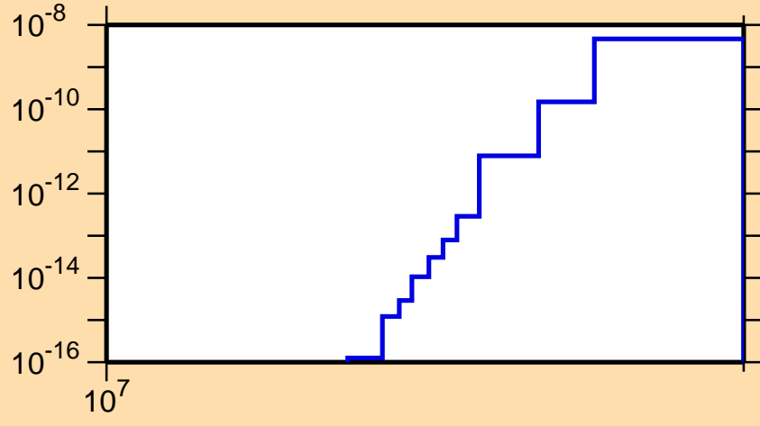
\sigma vs. E for ^{167}\text{Hf}(n,\text{pt})
