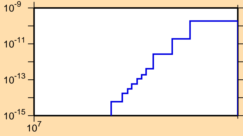
\sigma vs. E for ^{167}\text{Hf}(\text{mt117})
