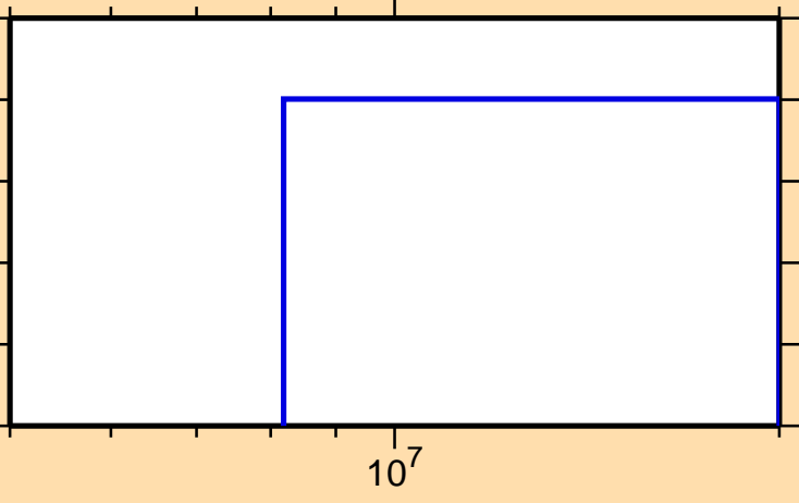
\sigma vs. E for ^{167}\text{Hf}(n,3n)
