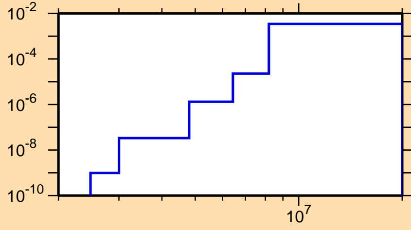
\sigma vs. E for ^{167}\text{Hf}(n,n\alpha)
