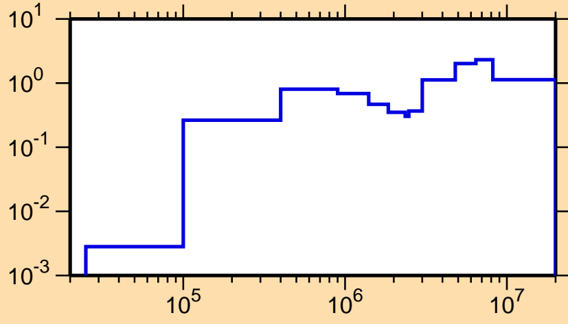
\sigma vs. E for ^{167}\text{Hf}(n,\text{inel.})
