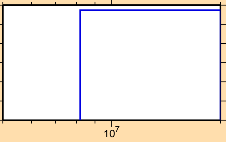
\sigma vs. E for ^{167}\text{Hf}(n,\text{pd})
