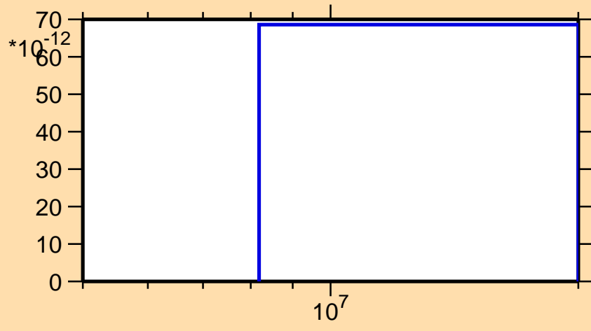
\sigma vs. E for ^{167}\text{Hf(mt 45)}
