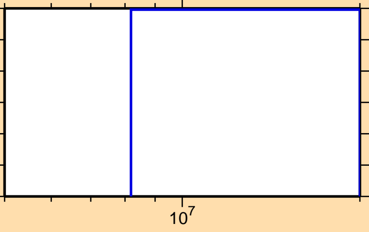
\sigma vs. E for ^{167}\text{Hf}(n,\text{nd})
