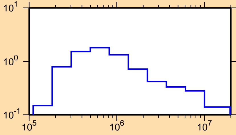
\sigma vs. E for ^{168}\text{Hf}(n,n_1)
