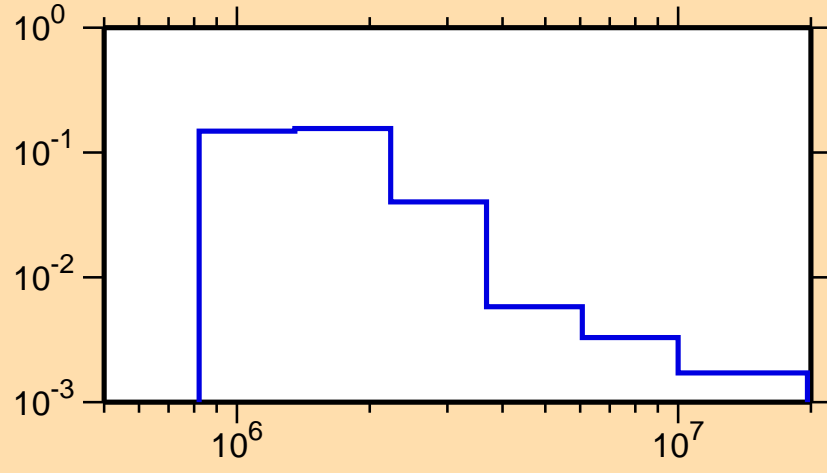
\sigma vs. E for ^{168}\text{Hf}(n,n_4)
