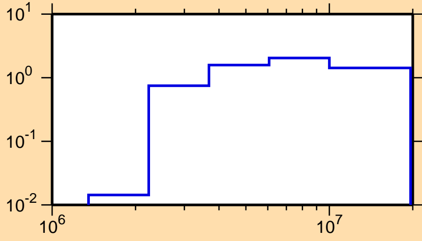
\sigma vs. E for ^{168}\text{Hf}(n,n\text{cont.})
