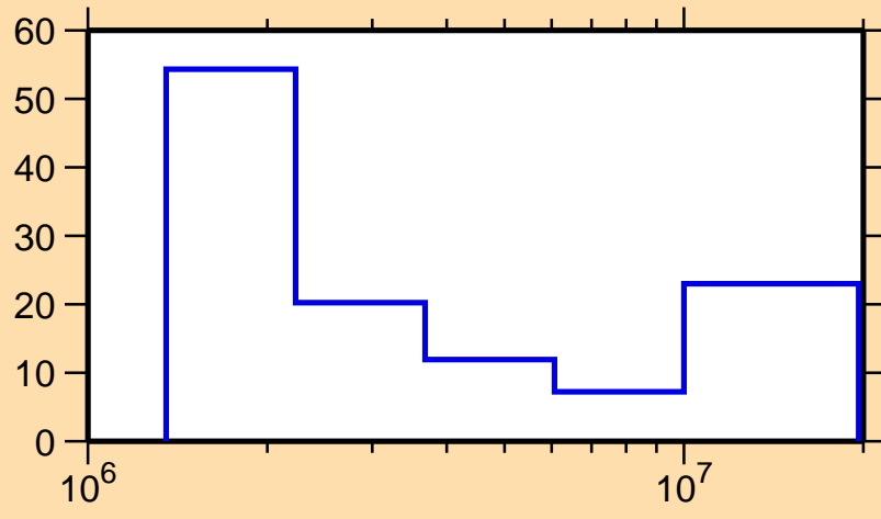
\Delta\sigma/\sigma vs. E for ^{168}\text{Hf}(n,n\text{cont.})
