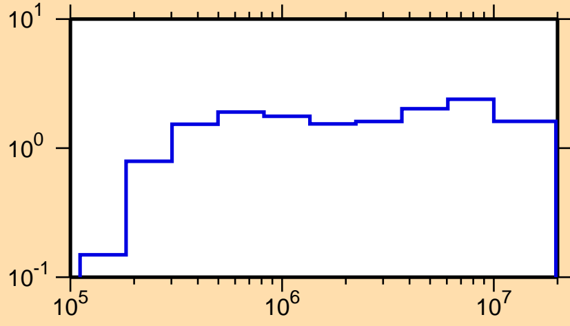
\sigma vs. E for ^{168}\text{Hf}(n,\text{inel.})
