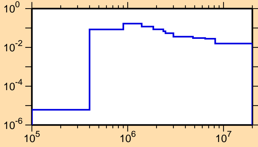
\sigma vs. E for ^{168}\text{Hf}(n,n_2)
