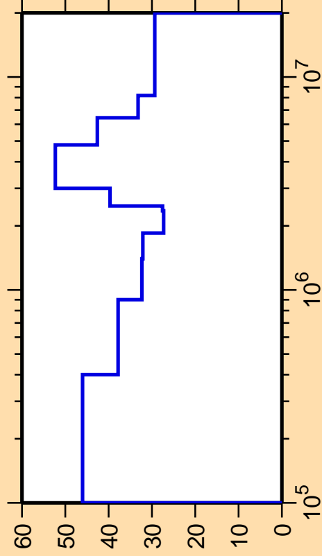
\Delta\sigma/\sigma vs. E for ^{168}\text{Hf}(n,n_2)
