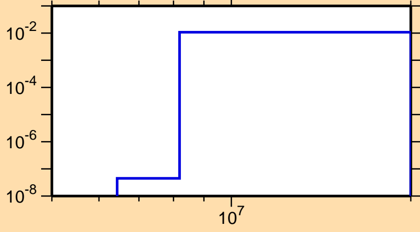
\sigma vs. E for ^{168}\text{Hf}(n,np)
