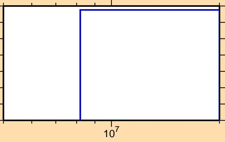
\sigma vs. E for ^{168}\text{Hf}(n,3n)
