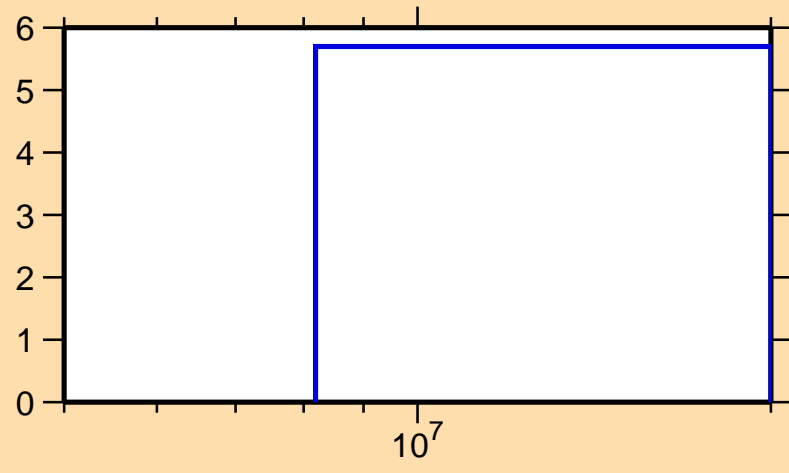
\Delta\sigma/\sigma vs. E for ^{168}\text{Hf}(n,\text{el.})
