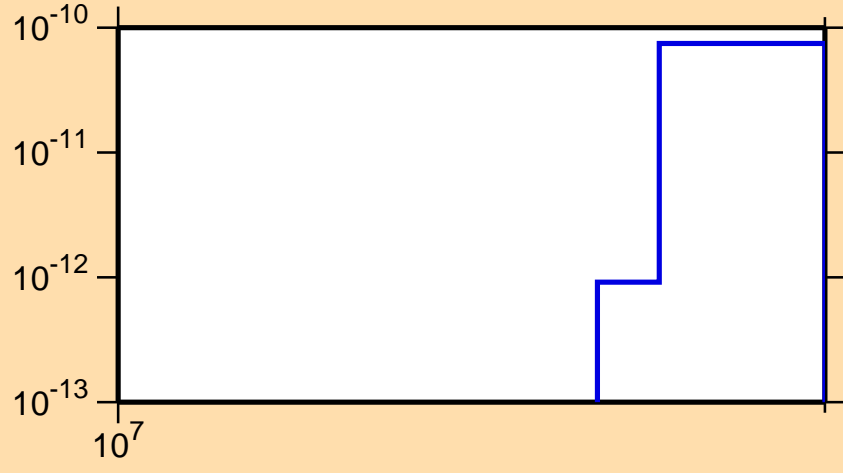
\sigma vs. E for ^{169}\text{Hf} (mt 34)
