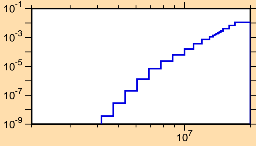
\sigma vs. E for ^{169}\text{Hf}(n,n\alpha)
