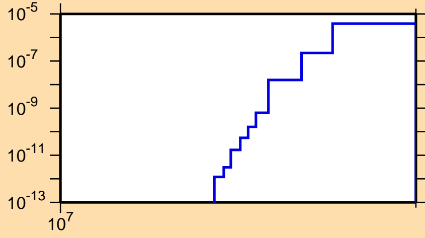
\sigma vs. E for ^{169}\text{Hf}(n,\text{nd})
