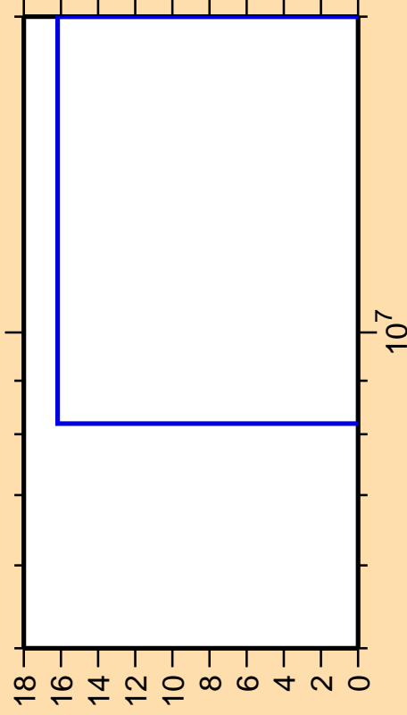
\Delta\sigma/\sigma vs. E for ^{169}\text{Hf}(n,pt)
