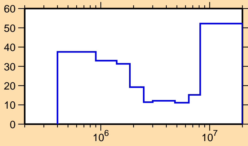
\Delta\sigma/\sigma vs. E for ^{169}\text{Hf}(n,n\text{cont.})
