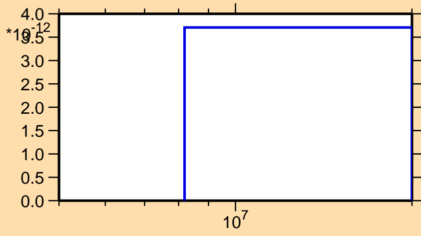
\sigma vs. E for ^{169}\text{Hf}(n,pt)
