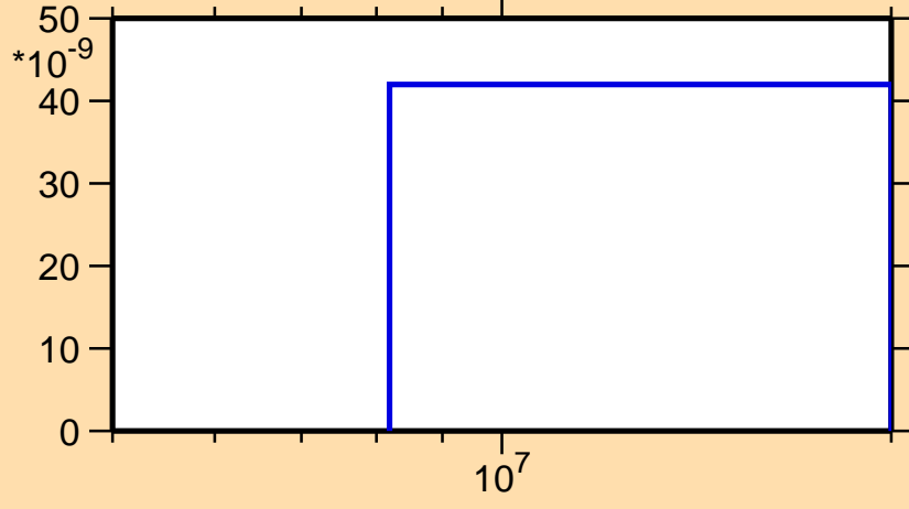
\sigma vs. E for ^{169}\text{Hf}(n,\text{nd})
