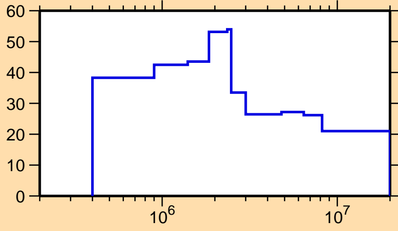
\Delta\sigma/\sigma vs. E for ^{169}\text{Hf}(n,n_1)
