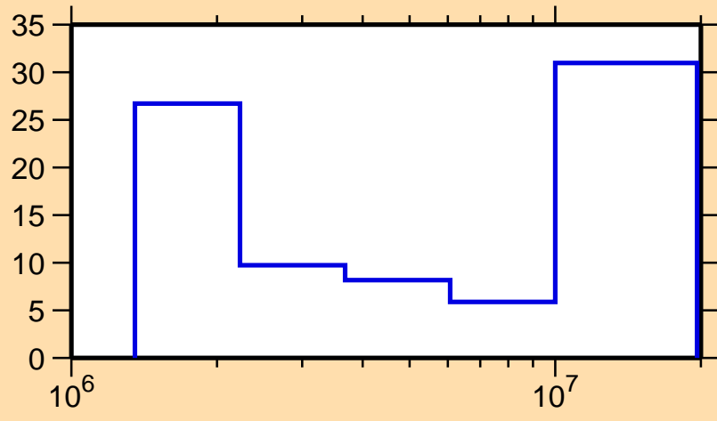
\Delta\sigma/\sigma vs. E for ^{170}\text{Hf}(n,ncont.)
