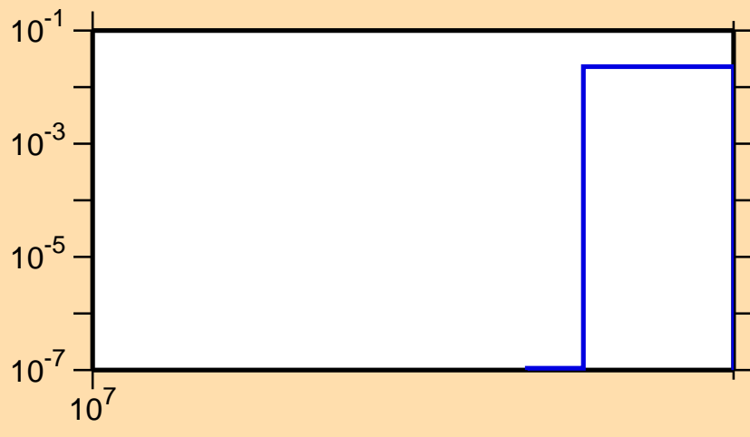
\sigma vs. E for ^{171}\text{Hf}(n,3n)
