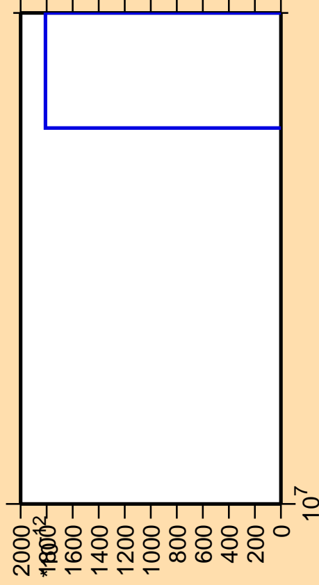
\Delta\sigma/\sigma vs. E for ^{171}\text{Hf} (mt 11)
