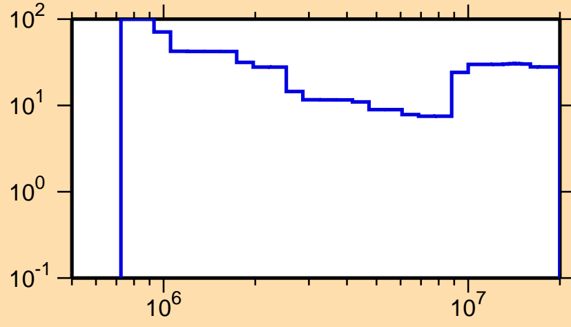
\Delta\sigma/\sigma vs. E for ^{171}\text{Hf}(n,n\text{cont.})
