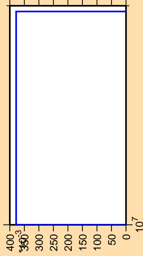
\Delta\sigma/\sigma vs. E for ^{171}\text{Hf}(\text{mt } 34)
