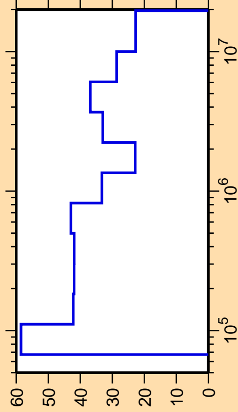
\Delta\sigma/\sigma vs. E for ^{171}\text{Hf}(n,n_4)
