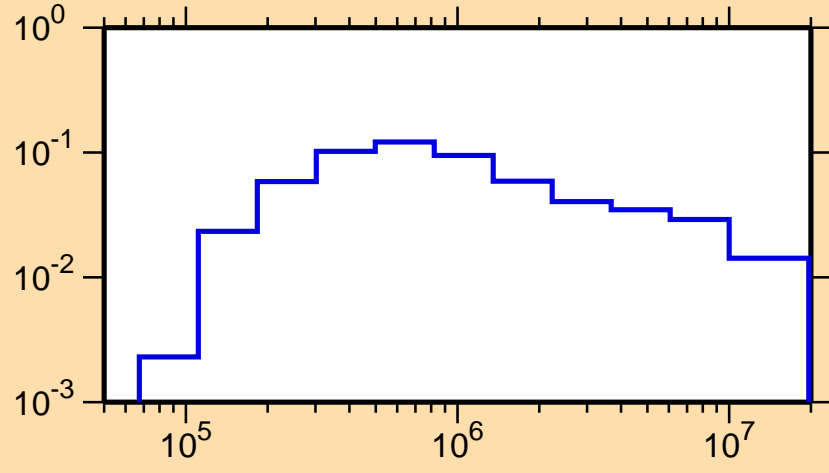
\sigma vs. E for ^{171}\text{Hf}(n,n_4)
