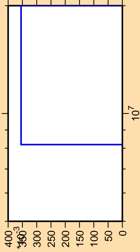
\Delta\sigma/\sigma vs. E for ^{171}\text{Hf}(n,\text{pt})
