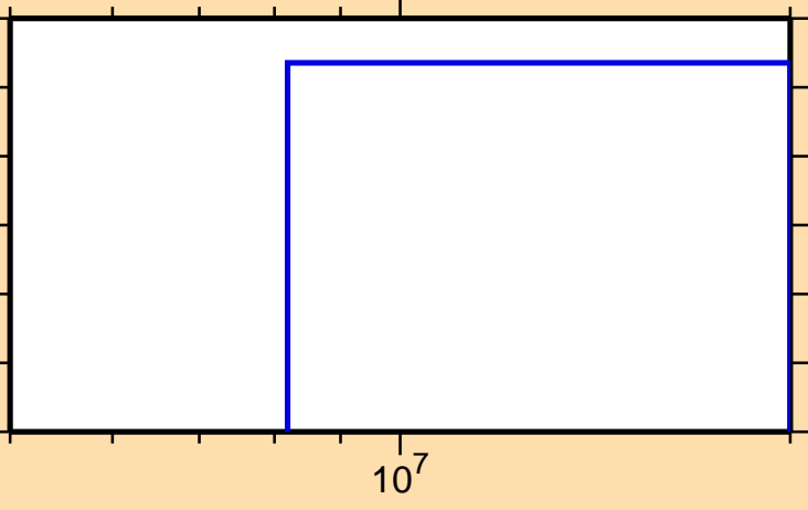
\sigma vs. E for ^{171}\text{Hf}(n,\text{nd})
