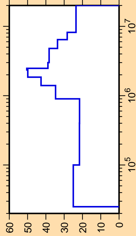
\Delta\sigma/\sigma vs. E for ^{171}\text{Hf}(n,n_2)
