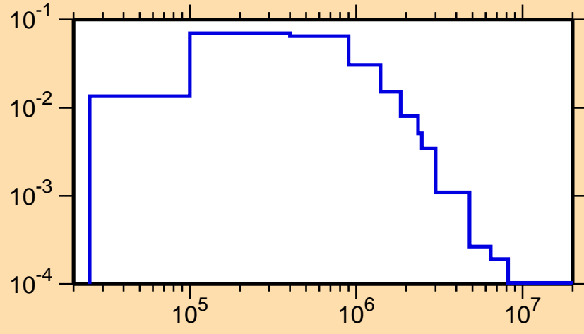
\sigma vs. E for ^{171}\text{Hf}(n,n_2)
