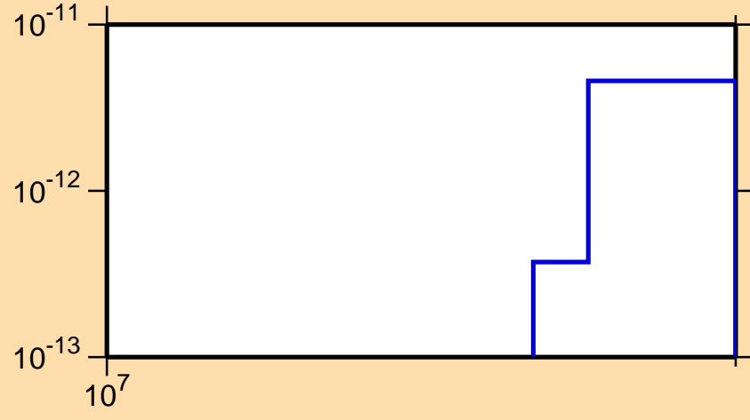
\sigma vs. E for ^{171}\text{Hf}(\text{mt117})
