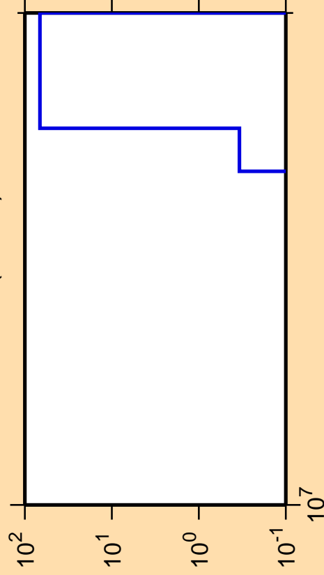
\Delta\sigma/\sigma vs. E for ^{171}\text{Hf} (mt 34)
