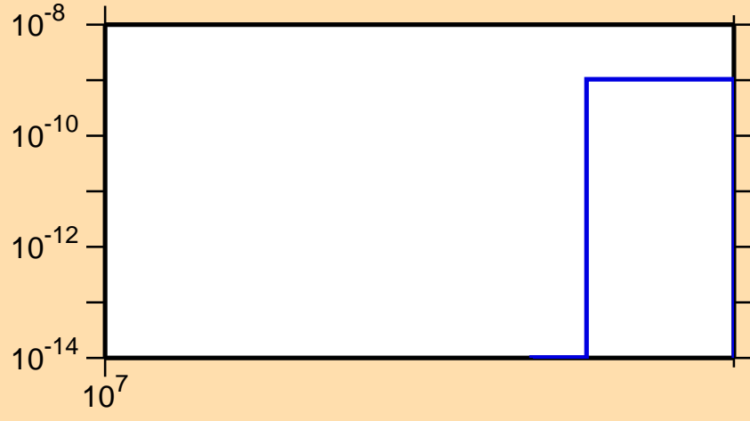
\sigma vs. E for ^{171}\text{Hf}(n,nt)
