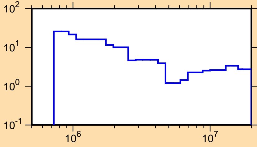
\Delta\sigma/\sigma vs. E for ^{171}\text{Hf}(n,n\text{onel.})
