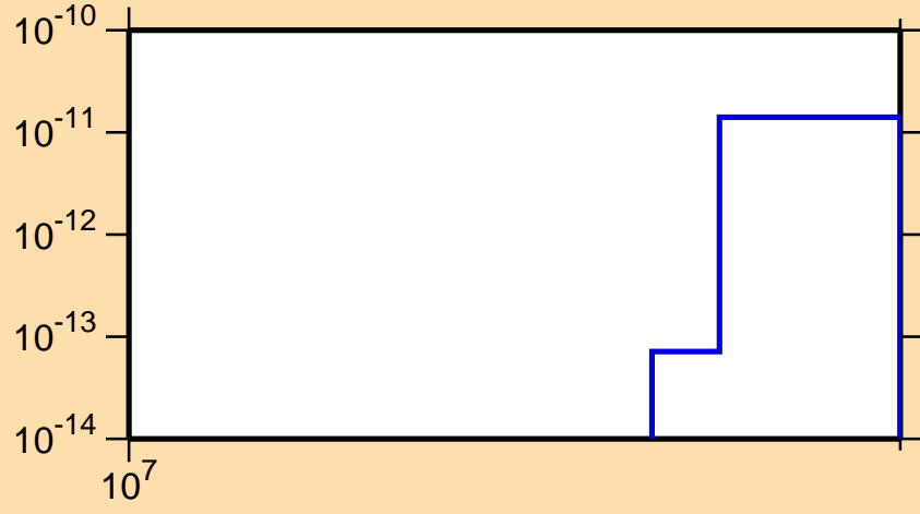
\sigma vs. E for ^{171}\text{Hf} (mt 34)
