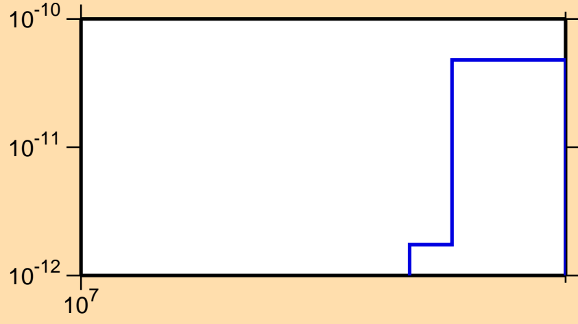
\sigma vs. E for ^{171}\text{Hf}(n,\text{pd})
