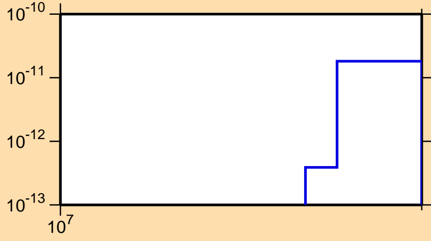
\sigma vs. E for ^{172}\text{Hf}(n,\text{pd})
