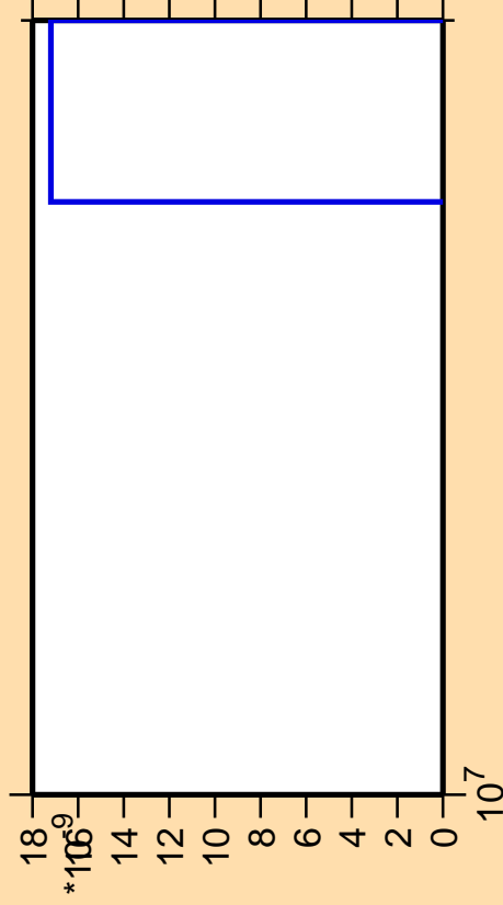
\Delta\sigma/\sigma vs. E for ^{172}\text{Hf} (mt 11)
