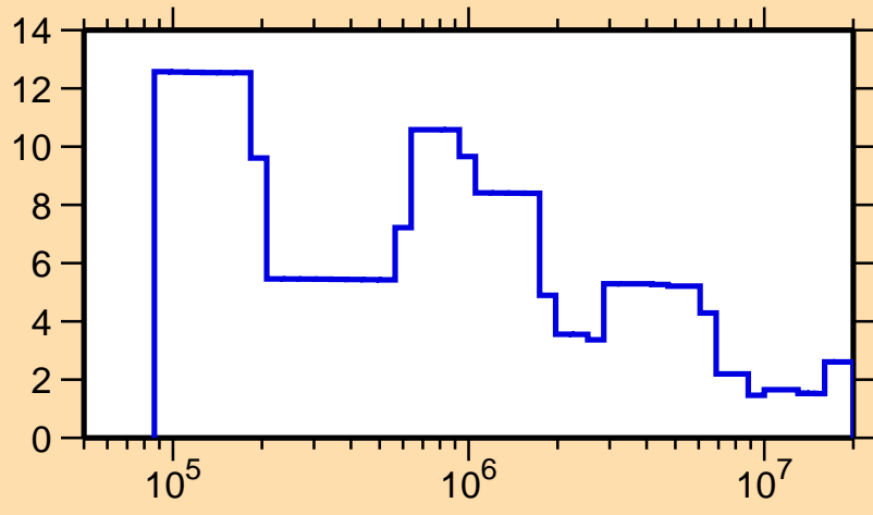
\Delta\sigma/\sigma vs. E for ^{172}\text{Hf}(n,\text{tot.})
