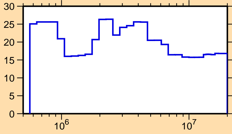
\Delta\sigma/\sigma vs. E for ^{172}\text{Hf}(n,n_1)
