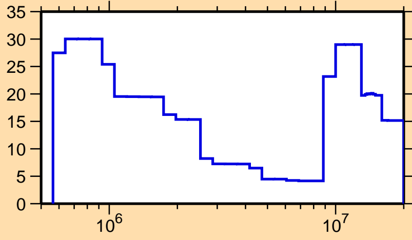
\Delta\sigma/\sigma vs. E for ^{172}\text{Hf}(n,\text{inel.})
