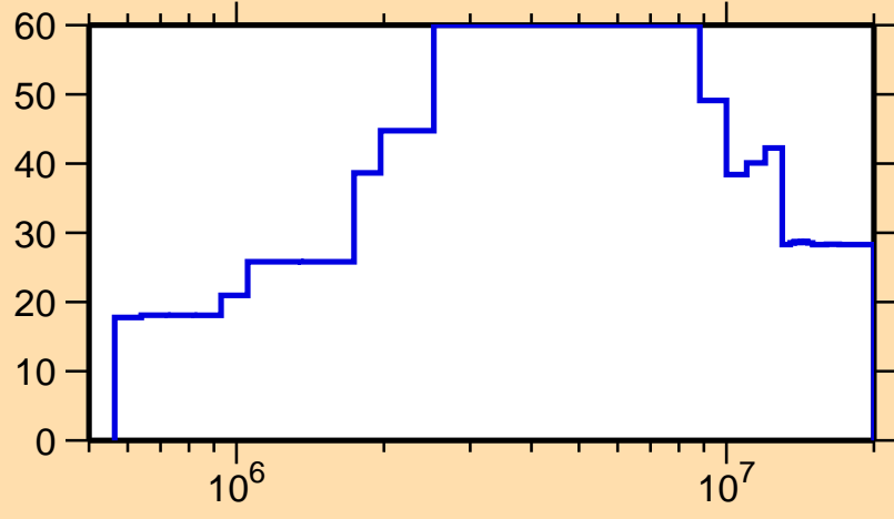
\Delta\sigma/\sigma vs. E for ^{172}\text{Hf}(n,\gamma)
