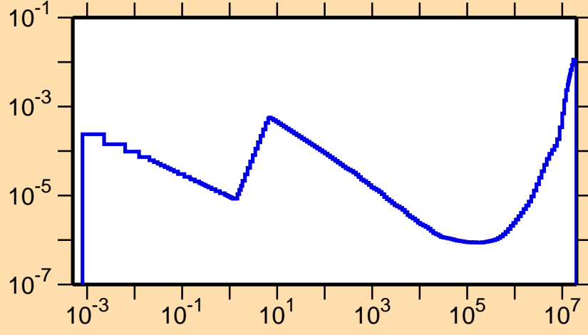
\sigma vs. E for ^{172}\text{Hf}(n,\alpha)
