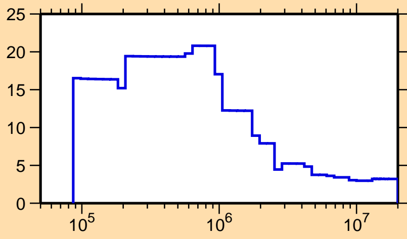
\Delta\sigma/\sigma vs. E for ^{172}\text{Hf}(n,\text{nonel.})
