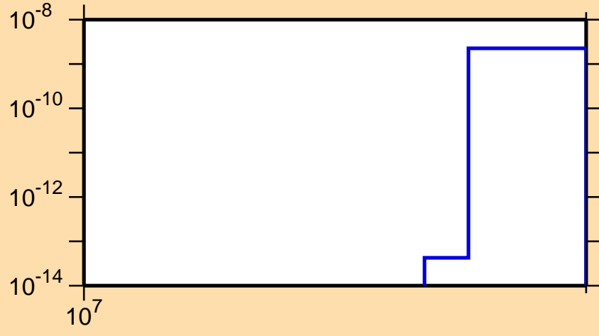
\sigma vs. E for ^{172}\text{Hf}(n,nt)
