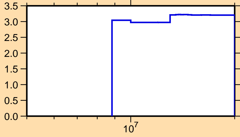
\Delta\sigma/\sigma vs. E for ^{172}\text{Hf}(n,\text{nonel.})
