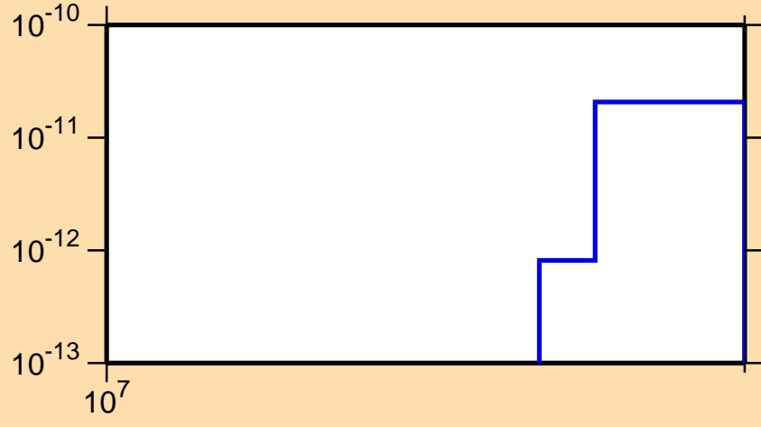
\sigma vs. E for ^{172}\text{Hf} (mt 45)
