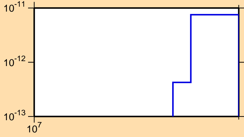
\sigma vs. E for ^{172}\text{Hf}(\text{mt117})
