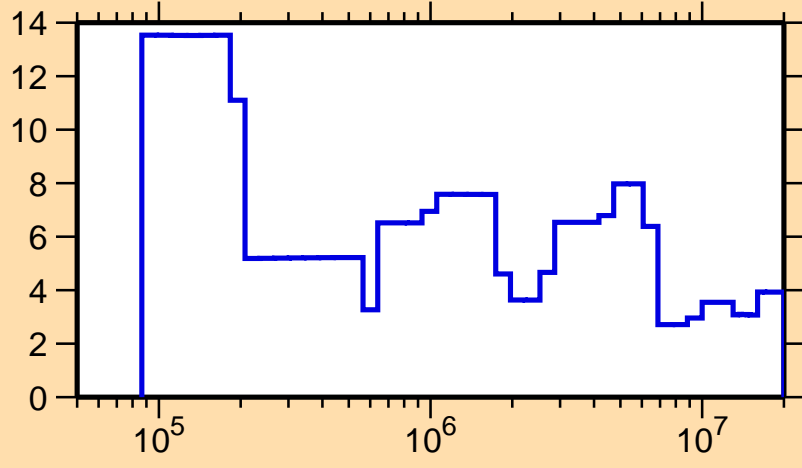
\Delta\sigma/\sigma vs. E for ^{172}\text{Hf}(n,\text{el.})
