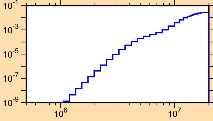
\sigma vs. E for ^{172}\text{Hf}(n,p)
