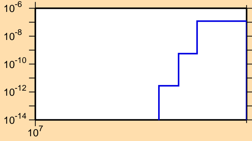
\sigma vs. E for ^{172}\text{Hf}(n,\text{nd})
