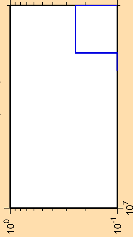
\Delta\sigma/\sigma vs. E for ^{172}\text{Hf}(\text{mt } 34)
