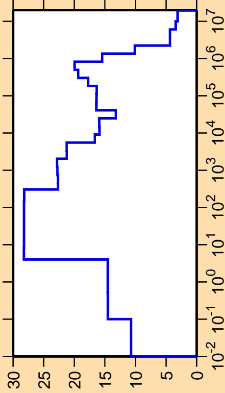
\Delta\sigma/\sigma vs. E for ^{172}\text{Hf}(n,\text{nonel.})
