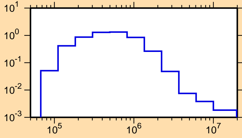
\sigma vs. E for ^{172}\text{Hf}(n,n_1)
