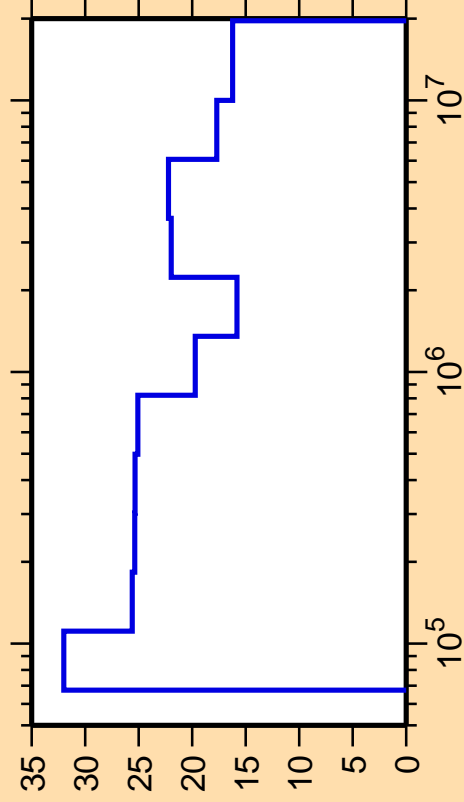
\Delta\sigma/\sigma vs. E for ^{172}\text{Hf}(n,n_1)
