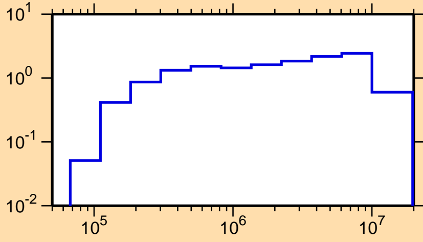
\sigma vs. E for ^{172}\text{Hf}(n,\text{inel.})
