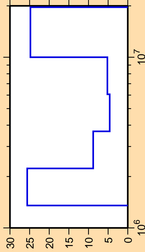
\Delta\sigma/\sigma vs. E for ^{172}\text{Hf}(n,\text{ncont.})
