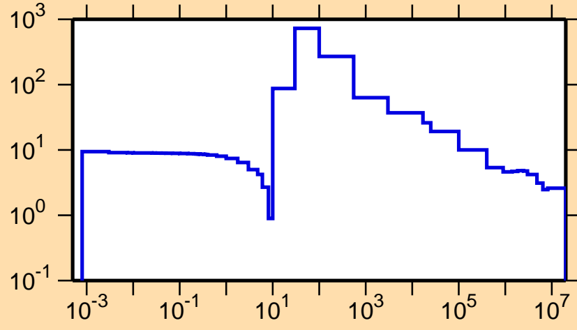
\sigma vs. E for ^{172}\text{Hf}(n,\text{el.})
