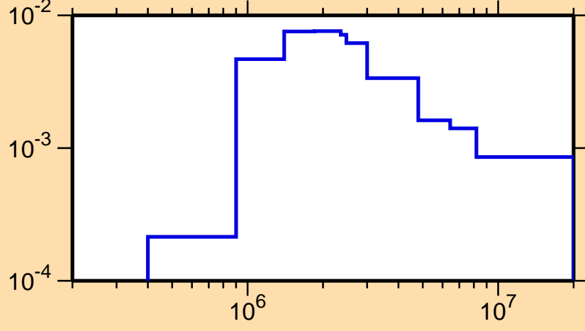
\sigma vs. E for ^{172}\text{Hf}(n,n_3)
