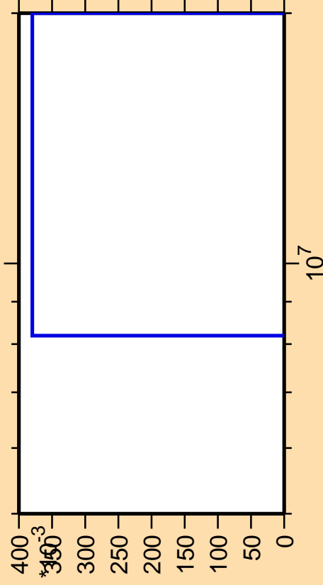
\Delta\sigma/\sigma vs. E for ^{172}\text{Hf}(n,pd)
