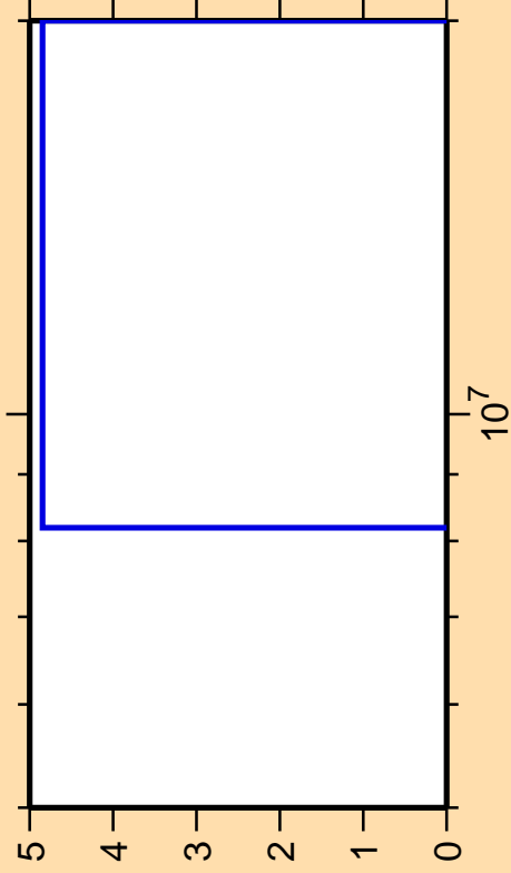
\Delta\sigma/\sigma vs. E for ^{172}\text{Hf}(n,2n)
