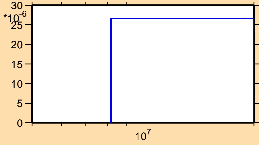
\sigma vs. E for ^{172}\text{Hf}(n,t)
