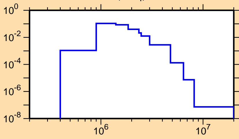
\sigma vs. E for ^{172}\text{Hf}(n,n_4)
