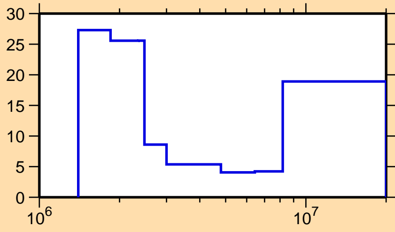
\Delta\sigma/\sigma vs. E for ^{172}\text{Hf}(n,n\text{cont.})
