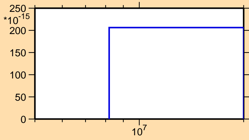
\sigma vs. E for ^{172}\text{Hf}(\text{mt } 45)
