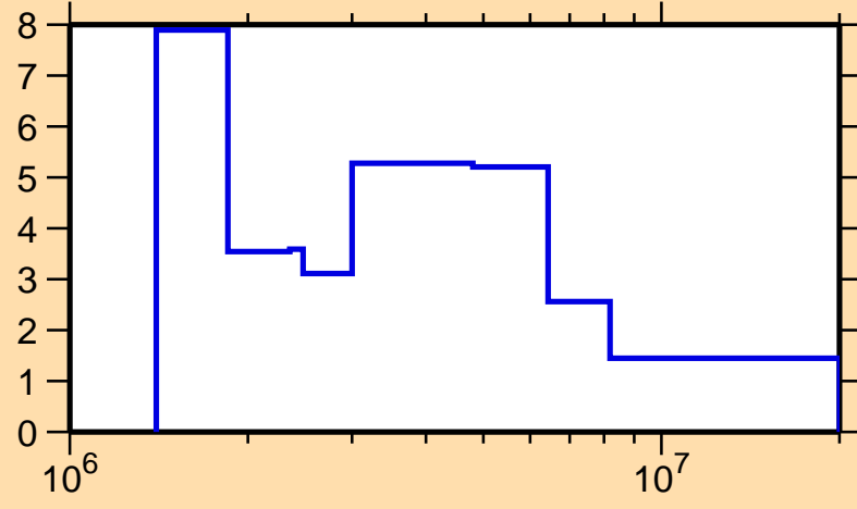
\Delta\sigma/\sigma vs. E for ^{172}\text{Hf}(n,\text{tot.})
