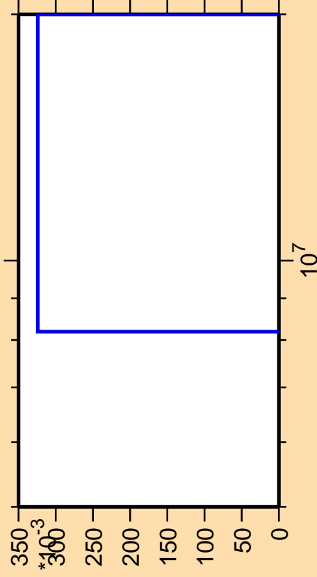
\Delta\sigma/\sigma vs. E for ^{172}\text{Hf}(\text{mt117})
