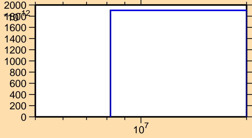
\sigma vs. E for ^{172}\text{Hf}(n,2np)
