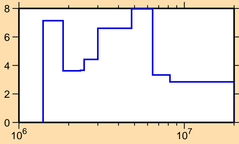
\Delta\sigma/\sigma vs. E for ^{172}\text{Hf}(n,el.)
