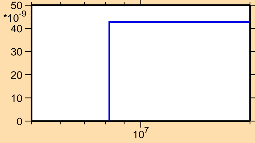
\sigma vs. E for ^{172}\text{Hf}(n,2n\alpha)
