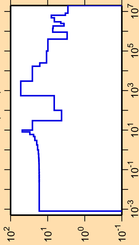
\Delta\sigma/\sigma vs. E for ^{172}\text{Hf}(n,\text{el.})
