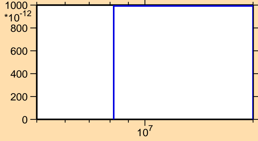
\sigma vs. E for ^{172}\text{Hf}(n,\text{nd})
