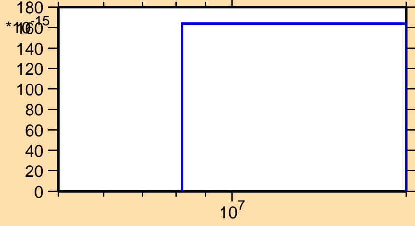
\sigma vs. E for ^{172}\text{Hf}(n,pd)
