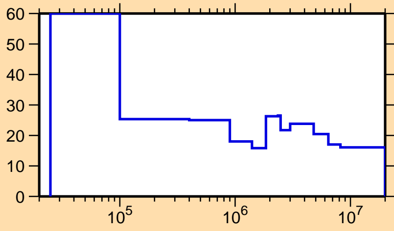
\Delta\sigma/\sigma vs. E for ^{172}\text{Hf}(n,n_1)
