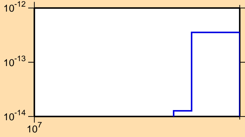
\sigma vs. E for ^{174}\text{Hf}(\text{mt117})
