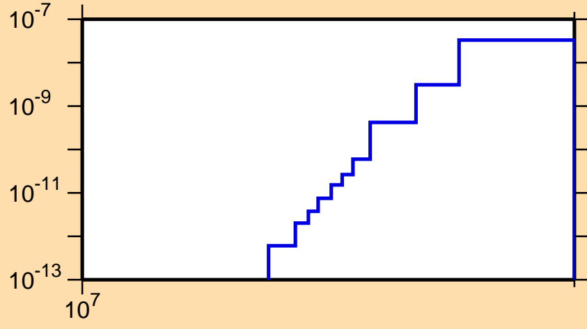
\sigma vs. E for ^{174}\text{Hf}(n,\text{He3})
