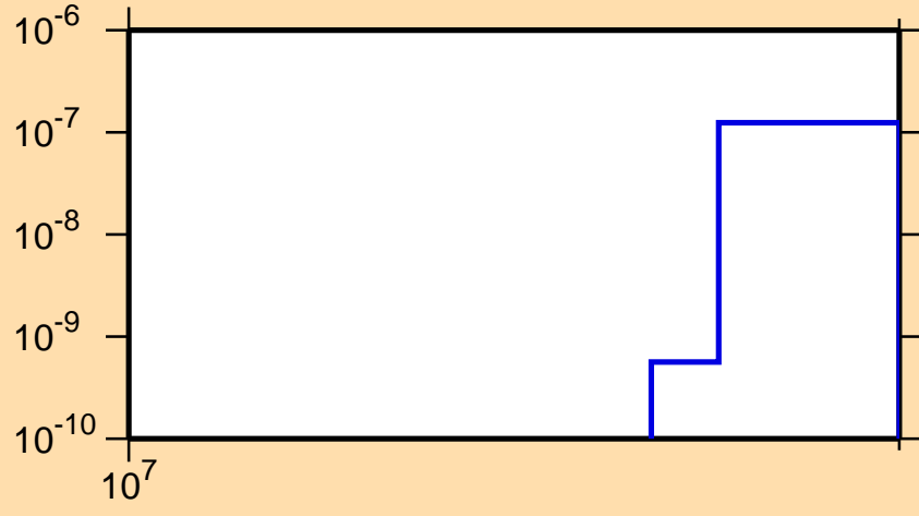
\sigma vs. E for ^{174}\text{Hf}(n,\text{nd})
