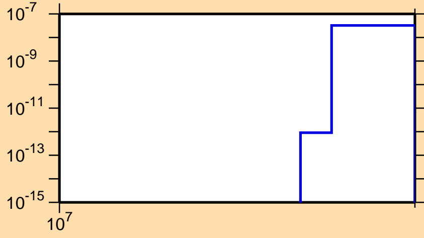
\sigma vs. E for ^{174}\text{Hf}(n,2np)
