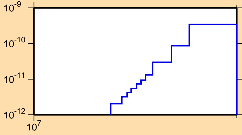
\sigma vs. E for ^{174}\text{Hf}(n,p\alpha)
