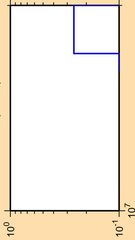
\Delta\sigma/\sigma vs. E for ^{174}\text{Hf} (mt 45)
