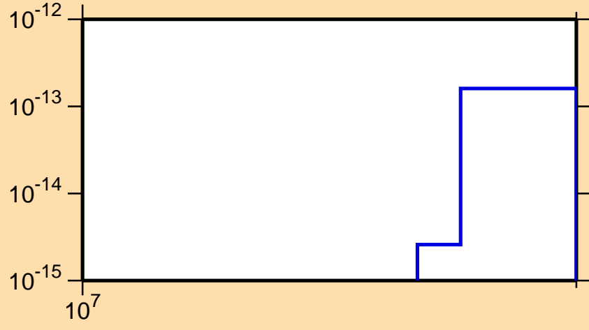
\sigma vs. E for ^{174}\text{Hf} (mt 45)
