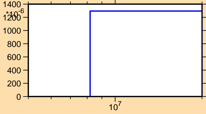
\sigma vs. E for ^{174}\text{Hf}(n,3n)
