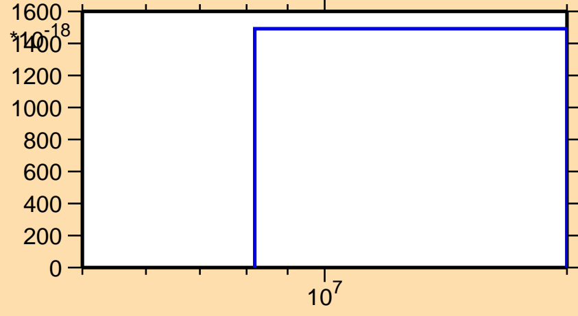
\sigma vs. E for ^{174}\text{Hf}(n,pd)
