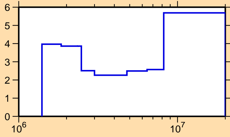
\Delta\sigma/\sigma vs. E for ^{174}\text{Hf}(n,n\text{cont.})
