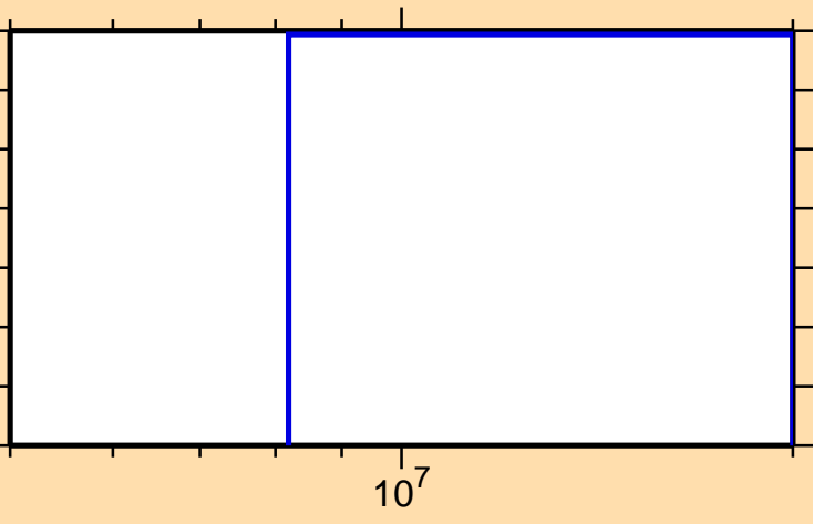
\sigma vs. E for ^{174}\text{Hf}(\text{mt117})
