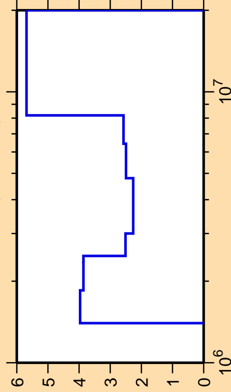
\Delta\sigma/\sigma vs. E for ^{174}\text{Hf}(n,n\text{cont.})
