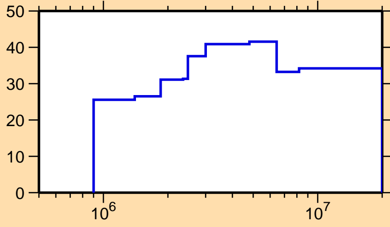
\Delta\sigma/\sigma vs. E for ^{174}\text{Hf}(n,\gamma)
