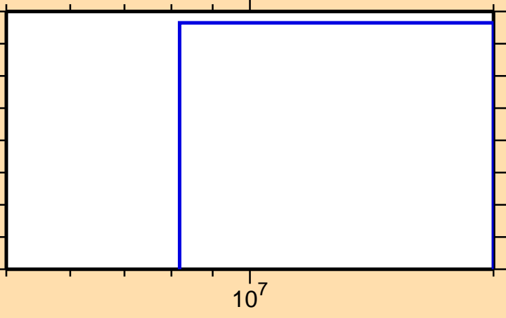
\sigma vs. E for ^{174}\text{Hf}(n,2n\alpha)
