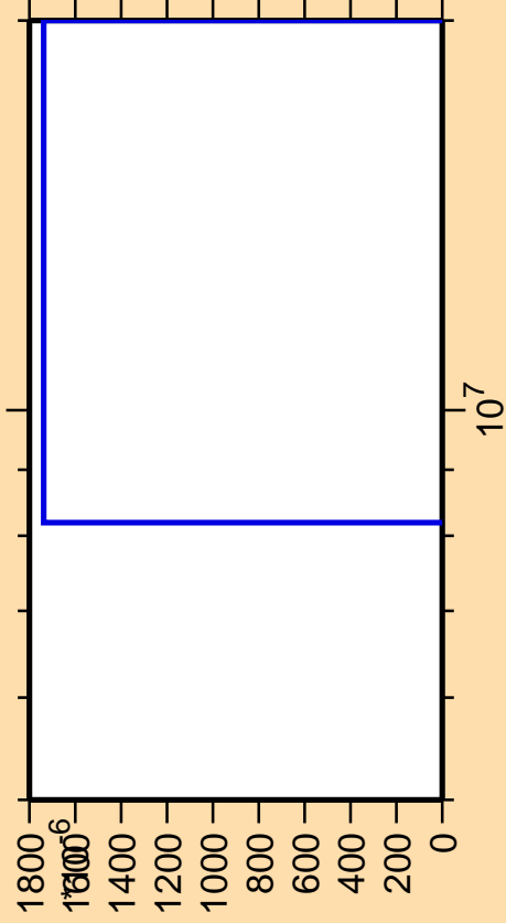
\Delta\sigma/\sigma vs. E for ^{174}\text{Hf}(n,pd)
