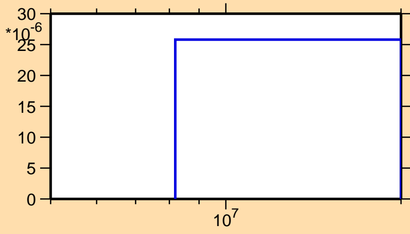
\sigma vs. E for ^{174}\text{Hf}(n,t)
