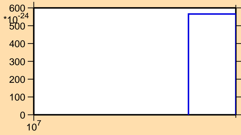
\sigma vs. E for ^{175}\text{Hf} (mt 11)
