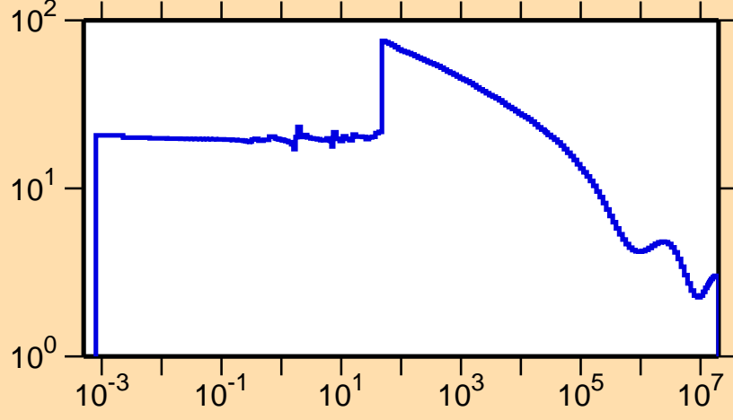
\sigma vs. E for ^{175}\text{Hf}(n,\text{el.})
