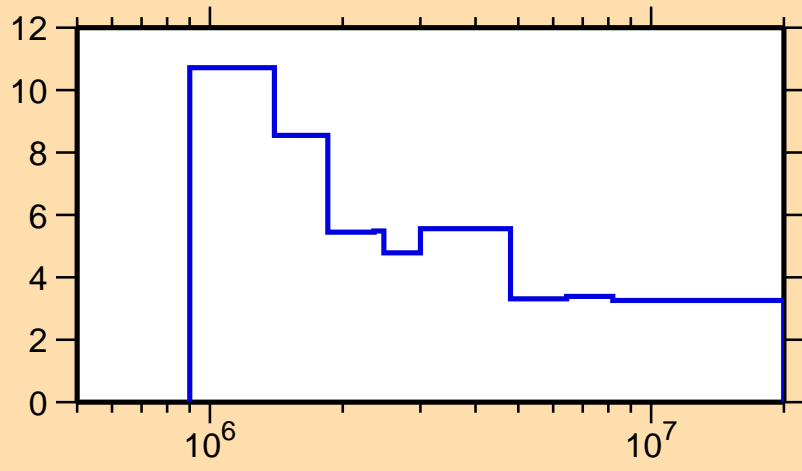
\Delta\sigma/\sigma vs. E for ^{175}\text{Hf}(n,n\text{onrel.})
