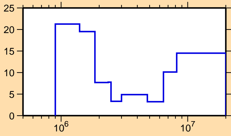
\Delta\sigma/\sigma vs. E for ^{175}\text{Hf}(n,ncont.)
