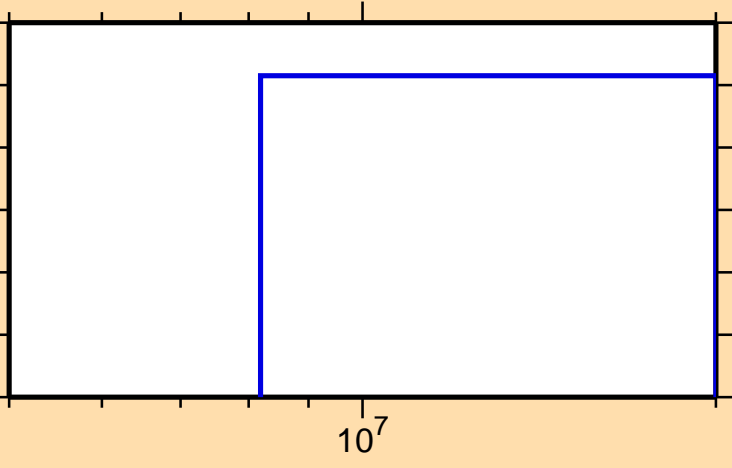
\sigma vs. E for ^{175}\text{Hf}(n,t)
