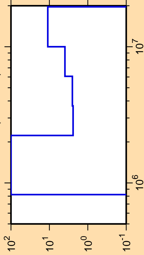
\Delta\sigma/\sigma vs. E for ^{177}\text{Hf}(n,\text{ncont.})
