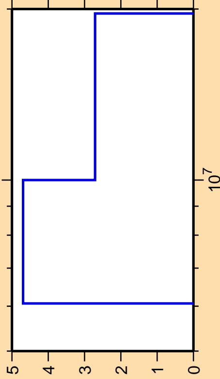
\Delta\sigma/\sigma vs. E for ^{177}\text{Hf}(n,2n)
