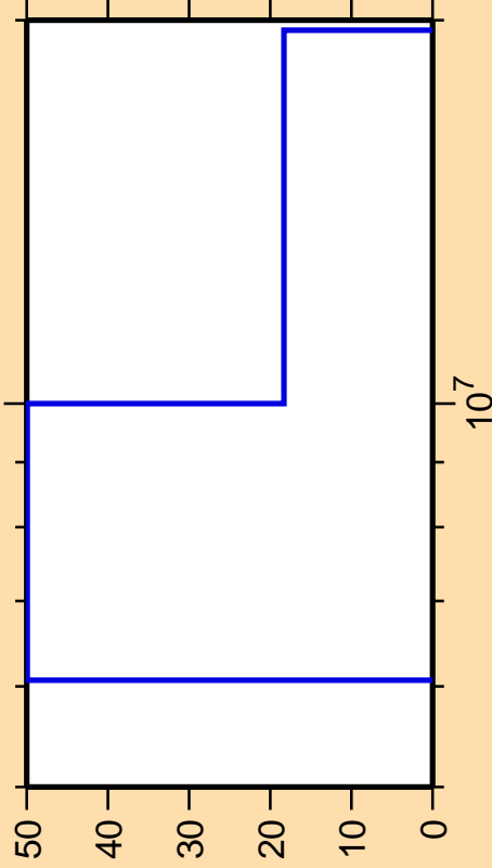
\Delta\sigma/\sigma vs. E for ^{177}\text{Hf}(n,np)
