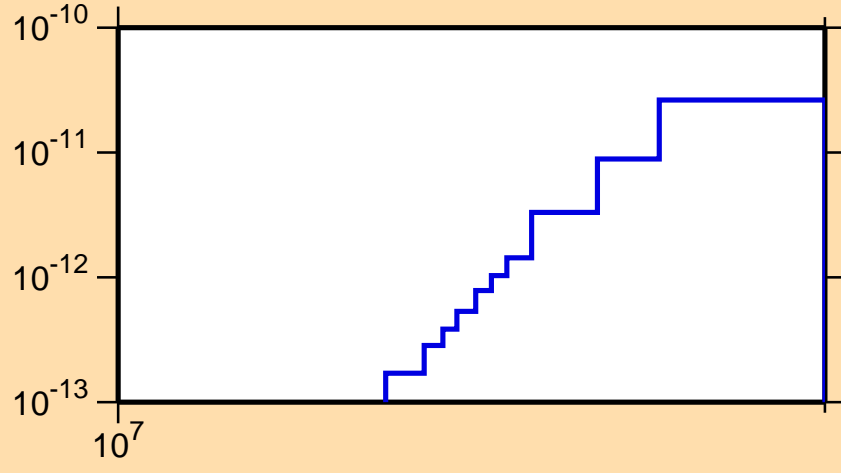
\sigma vs. E for ^{177}\text{Hf}(n,p\alpha)
