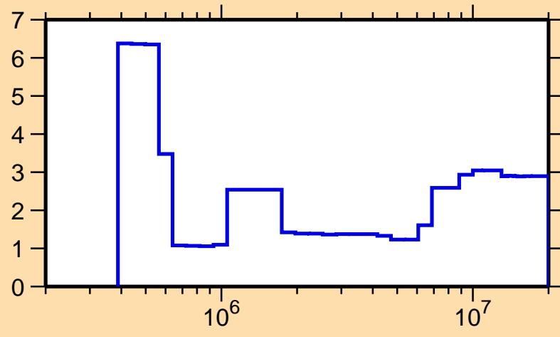
\Delta\sigma/\sigma vs. E for ^{178}\text{Hf}(n,n\text{onel.})
