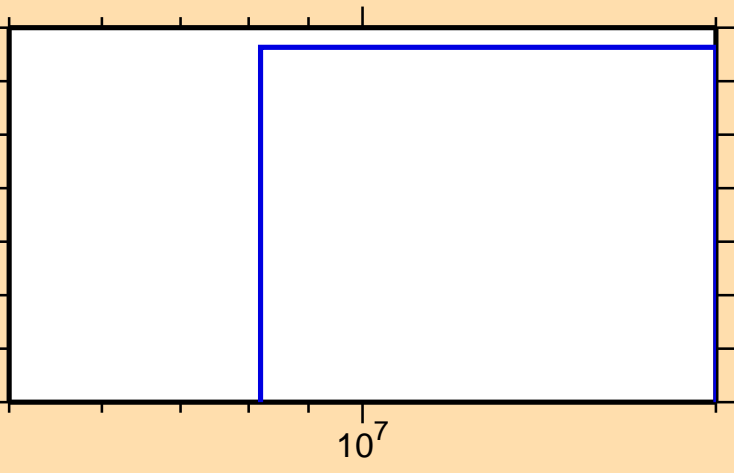
\sigma vs. E for ^{178}\text{Hf}(n,3n\alpha)
