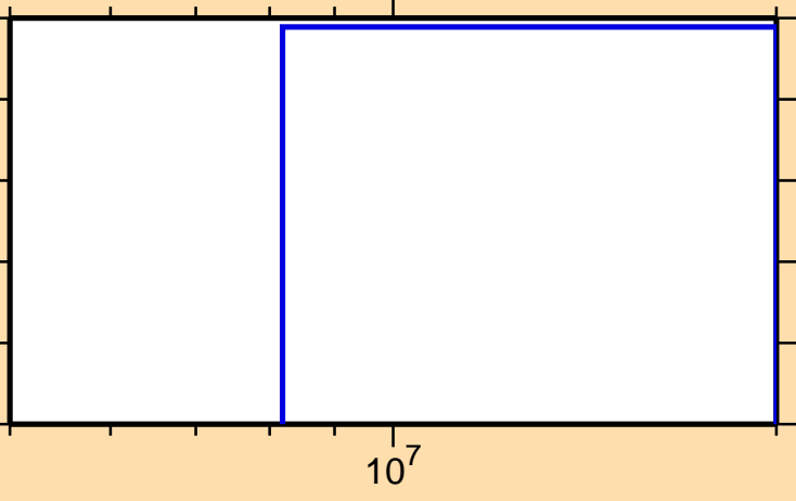
\sigma vs. E for ^{178}\text{Hf}(n,2n\alpha)
