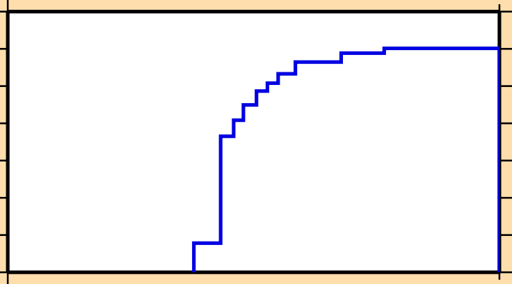
\sigma vs. E for ^{179}\text{Hf}(n,3n)
