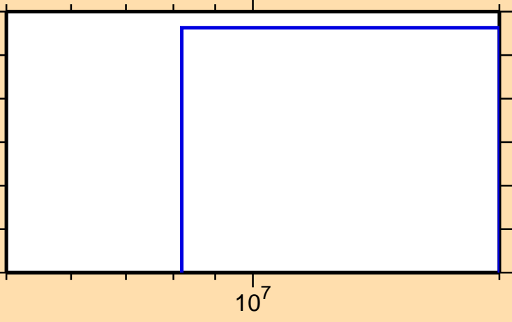
\sigma vs. E for ^{180}\text{Hf}(n,nt)
