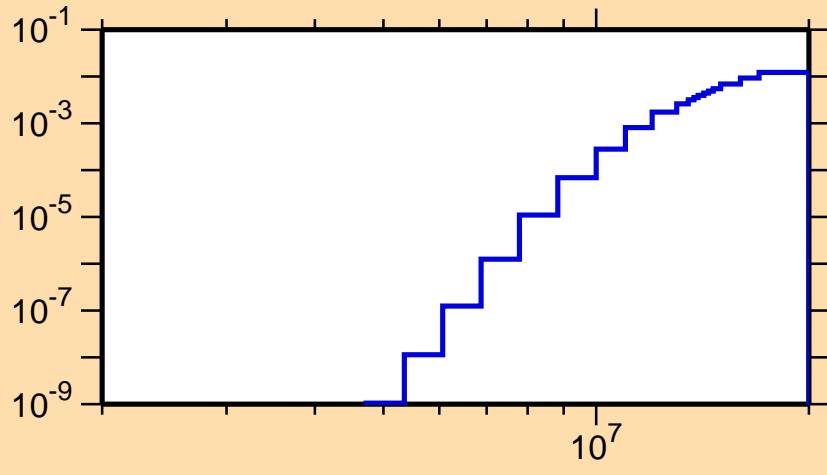
\sigma vs. E for ^{180}\text{Hf}(n,p)
