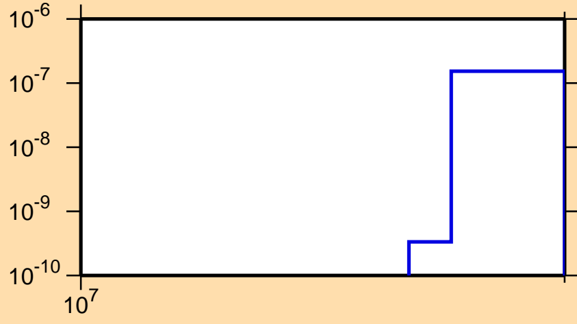
\sigma vs. E for ^{181}\text{Hf}(n,nt)
