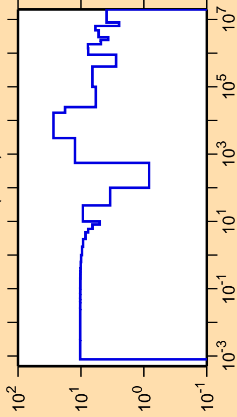
\Delta\sigma/\sigma vs. E for ^{181}\text{Hf}(n,\text{el.})
