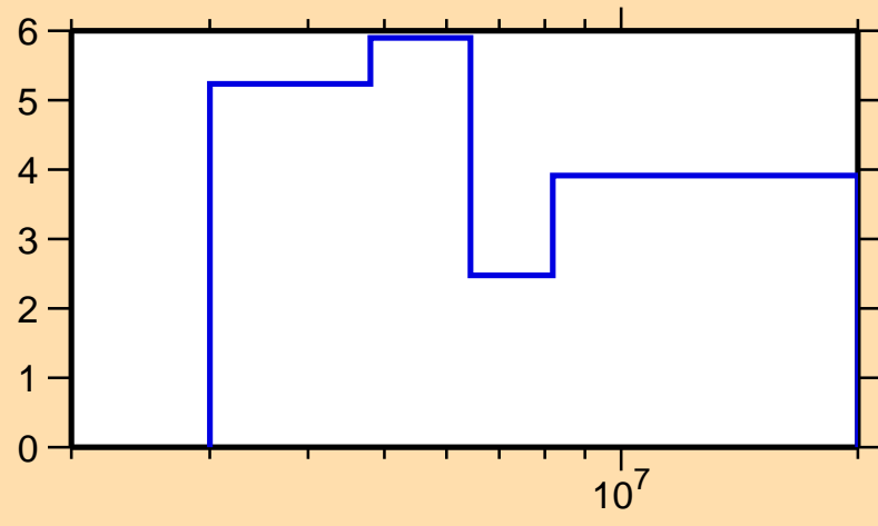
\Delta\sigma/\sigma vs. E for ^{181}\text{Hf}(n,\text{el.})
