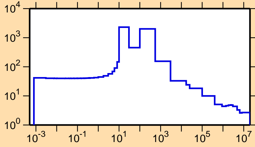
\sigma vs. E for ^{181}\text{Hf}(n,\text{el.})
