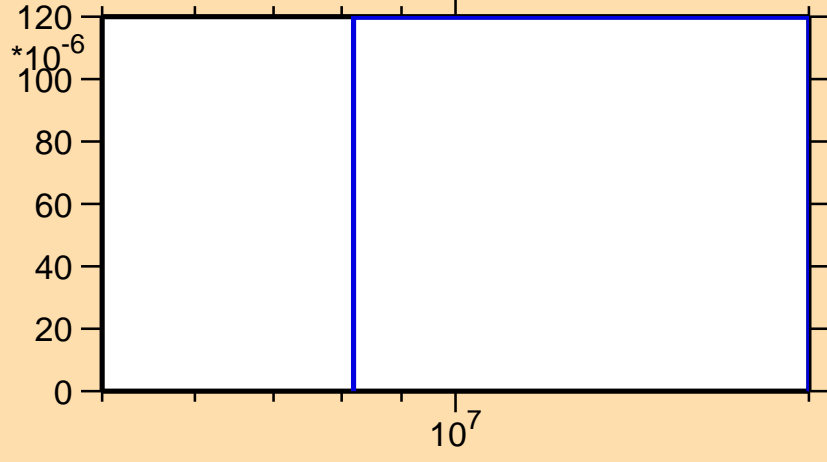
\sigma vs. E for ^{181}\text{Hf}(n,d)
