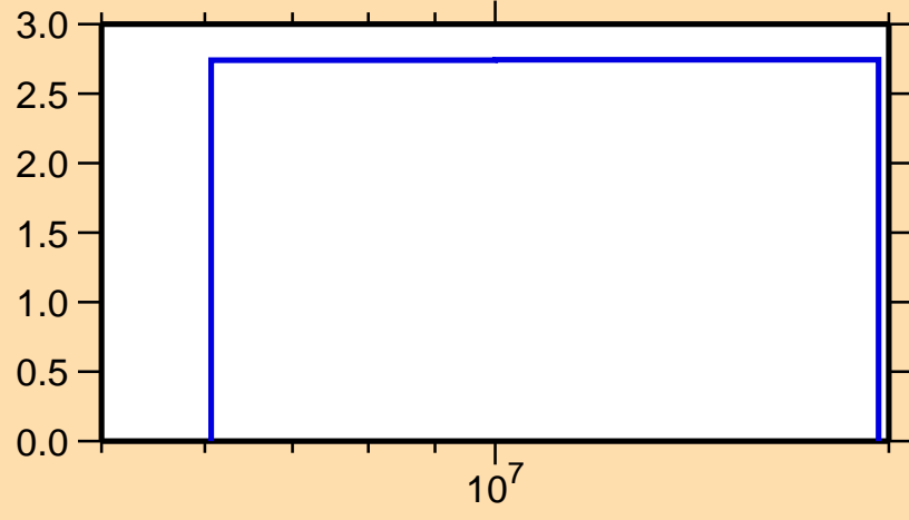
\Delta\sigma/\sigma vs. E for ^{182}\text{Hf}(n,el.)
