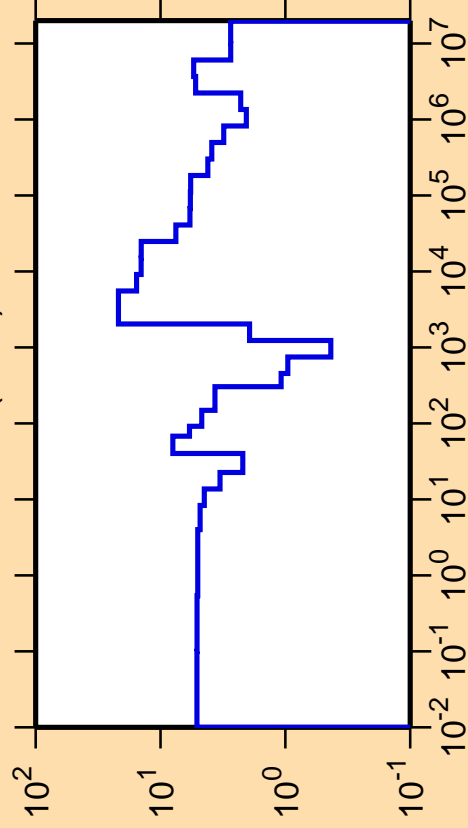
\Delta\sigma/\sigma vs. E for ^{182}\text{Hf}(n,\text{el.})
