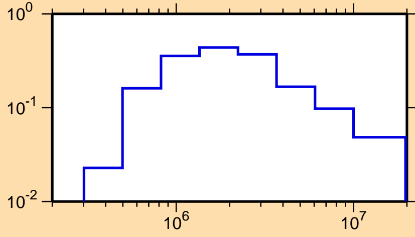
\sigma vs. E for ^{182}\text{Hf}(n,n_2)
