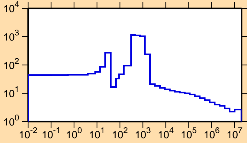
\sigma vs. E for ^{182}\text{Hf}(n,\text{el.})
