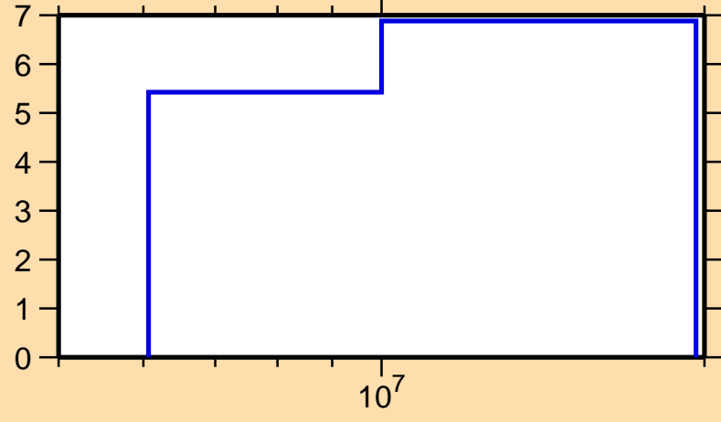
\Delta\sigma/\sigma vs. E for ^{182}\text{Hf}(n,2n)
