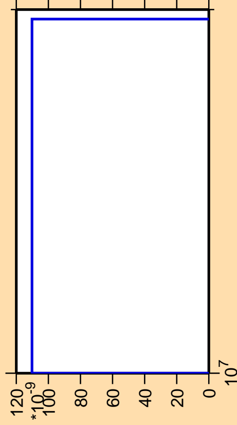
\Delta\sigma/\sigma vs. E for ^{182}\text{Hf} (mt 11)
