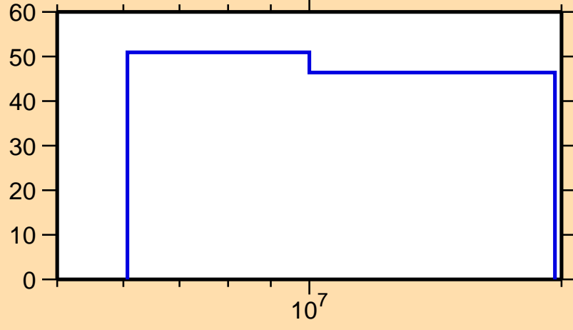
\Delta\sigma/\sigma vs. E for ^{182}\text{Hf}(n,p)
