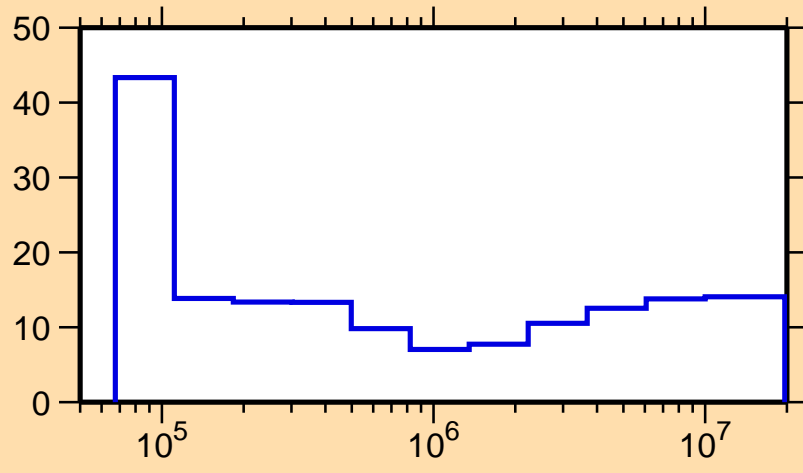
\Delta\sigma/\sigma vs. E for ^{182}\text{Hf}(n,n_1)
