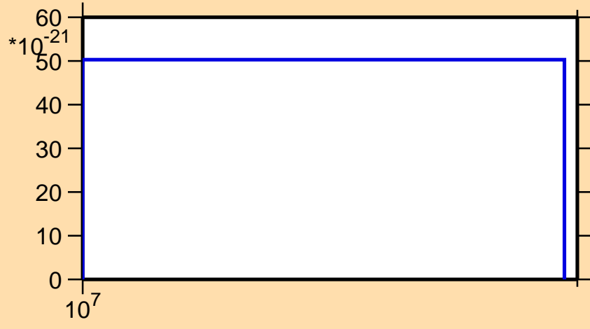
\sigma vs. E for ^{182}\text{Hf} (mt 11)
