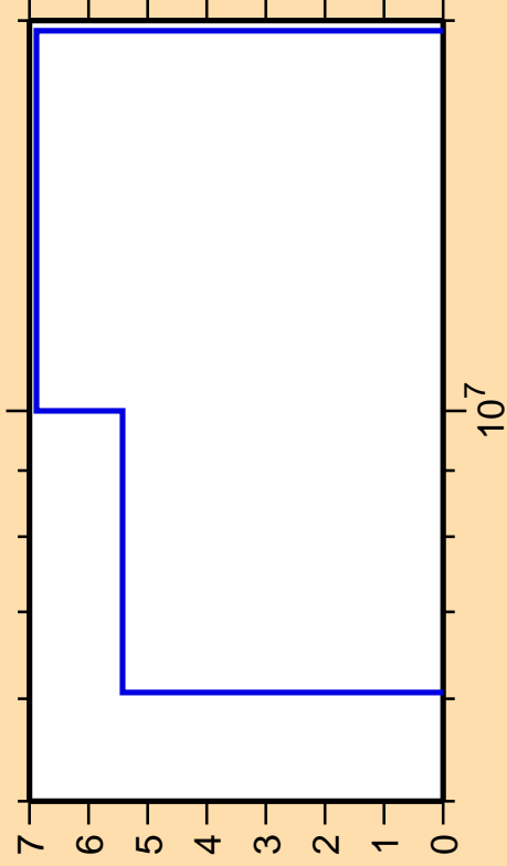
\Delta\sigma/\sigma vs. E for ^{182}\text{Hf}(n,2n)
