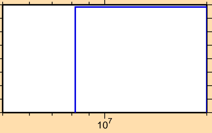
\sigma vs. E for ^{182}\text{Hf}(n,t)
