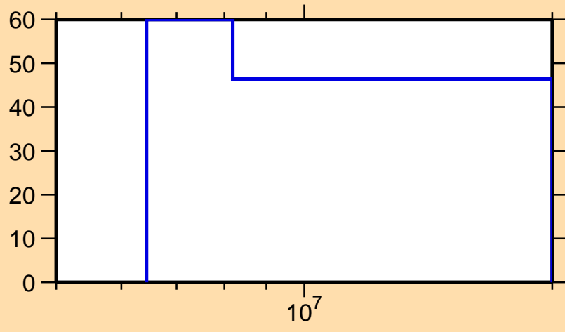
\Delta\sigma/\sigma vs. E for ^{182}\text{Hf}(n,p)
