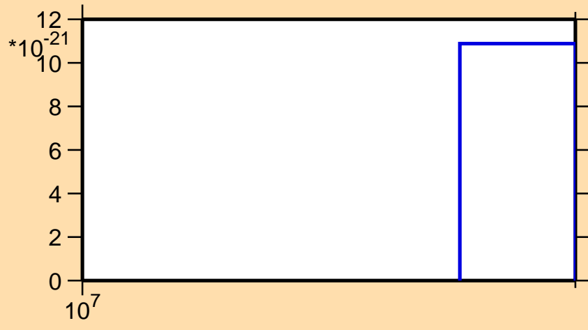
\sigma vs. E for ^{182}\text{Hf} (mt 42)
