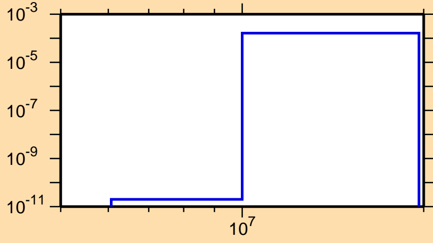
\sigma vs. E for ^{182}\text{Hf}(n,d)
