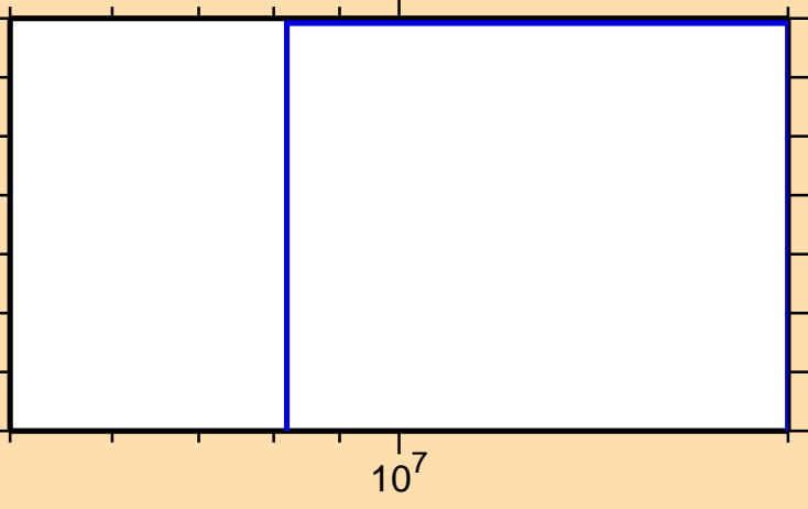
\sigma vs. E for ^{182}\text{Hf}(n,nt)
