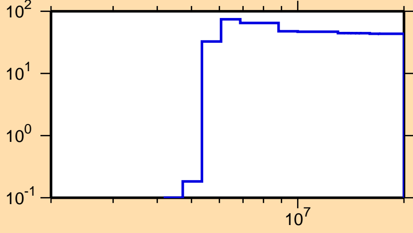
\Delta\sigma/\sigma vs. E for ^{183}\text{Hf}(n,p)
