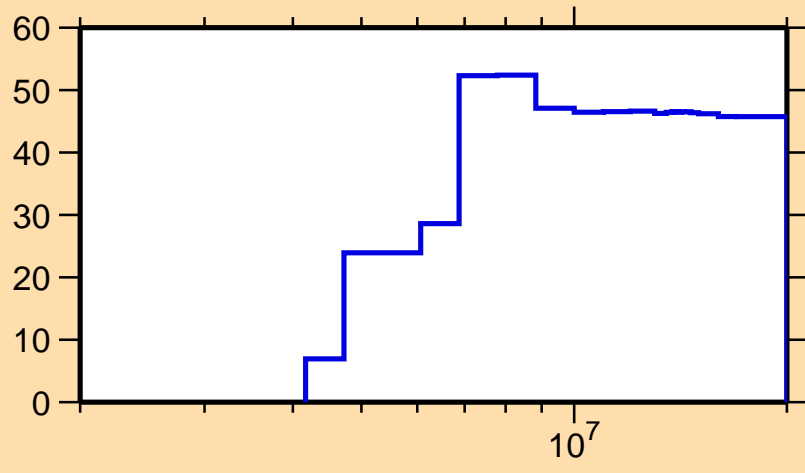
\Delta\sigma/\sigma vs. E for ^{183}\text{Hf}(n,n\text{cont.})
