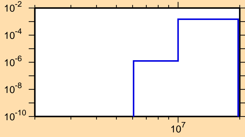
\sigma vs. E for ^{183}\text{Hf}(n,p)
