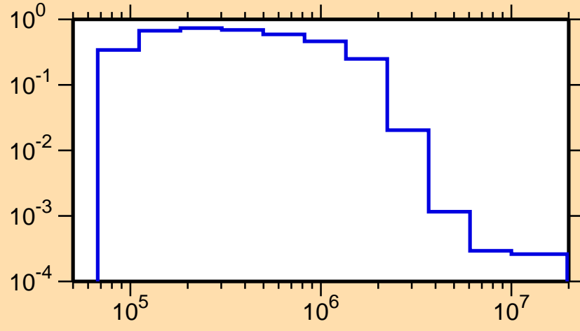
\sigma vs. E for ^{183}\text{Hf}(n,n_1)
