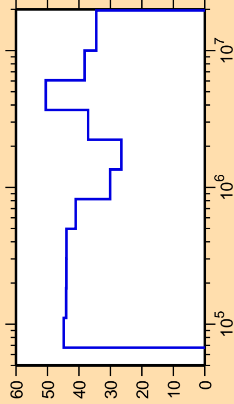
\Delta\sigma/\sigma vs. E for ^{183}\text{Hf}(n,n_1)
