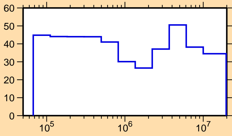
\Delta\sigma/\sigma vs. E for ^{183}\text{Hf}(n,n_1)
