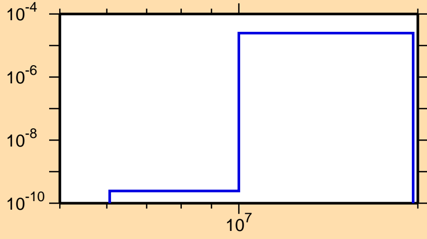
\sigma vs. E for ^{183}\text{Hf}(n,n\alpha)
