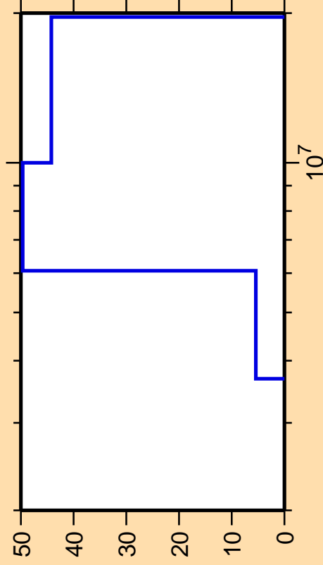
\Delta\sigma/\sigma vs. E for ^{183}\text{Hf}(n,p)
