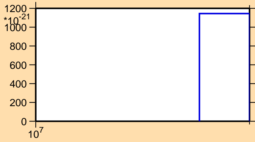
\sigma vs. E for ^{184}\text{Hf}(\text{mt } 42)
