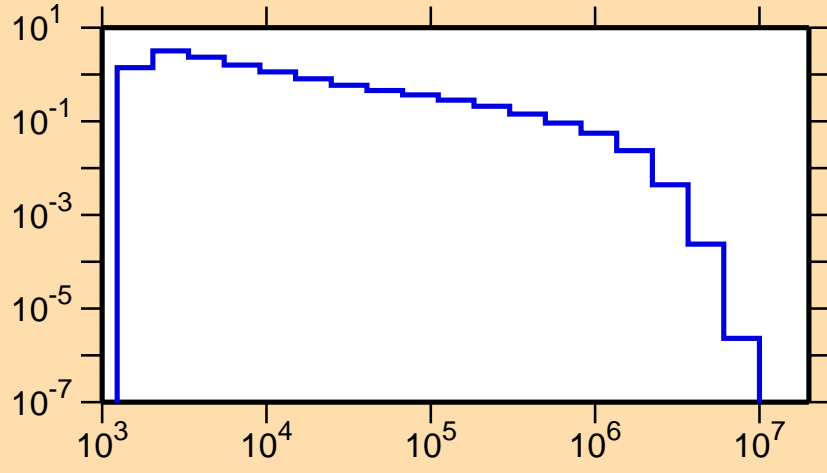
\sigma vs. E for ^{184}\text{Hf}(n,n_4)
