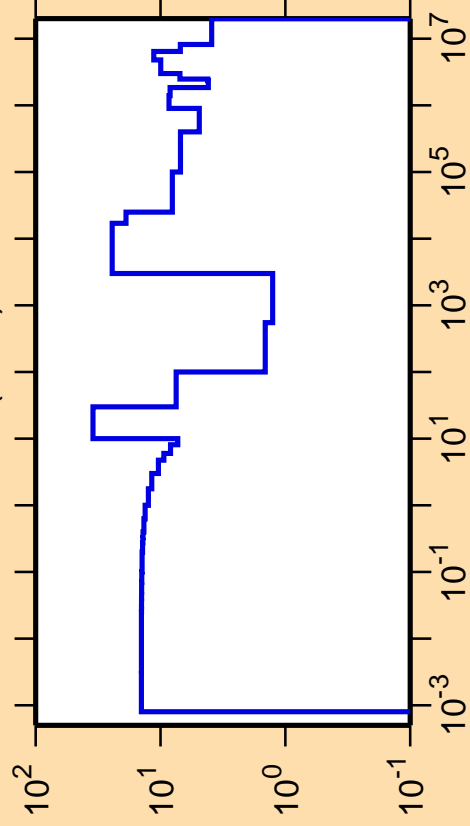
\Delta\sigma/\sigma vs. E for ^{184}\text{Hf}(n,\text{el.})
