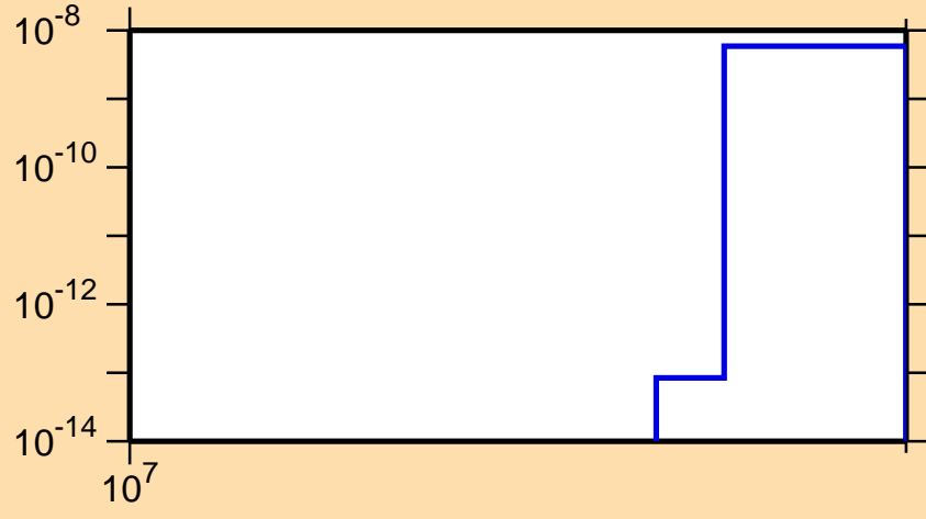
\sigma vs. E for ^{187}\text{Hf}(n,2np)
