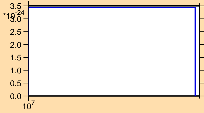
\sigma vs. E for ^{187}\text{Hf} (mt 11)
