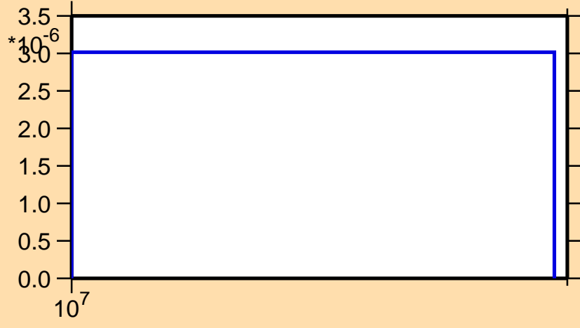
\sigma vs. E for ^{187}\text{Hf}(n,np)
