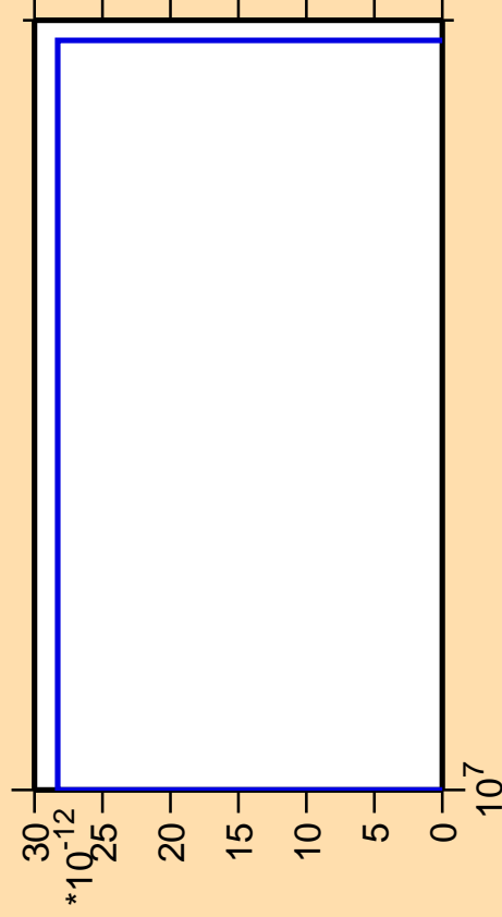
\Delta\sigma/\sigma vs. E for ^{187}\text{Hf} (mt 11)
