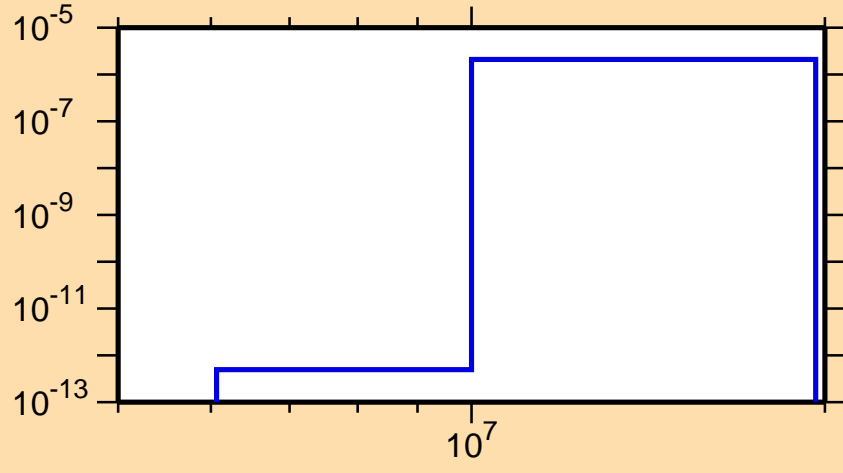
\sigma vs. E for ^{187}\text{Hf}(n,n\alpha)
