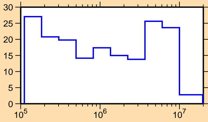
\Delta\sigma/\sigma vs. E for ^{187}\text{Hf}(n,el.)
