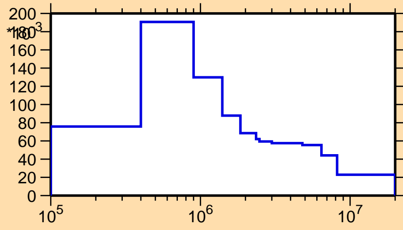
\sigma vs. E for ^{187}\text{Hf}(n,n_1)
