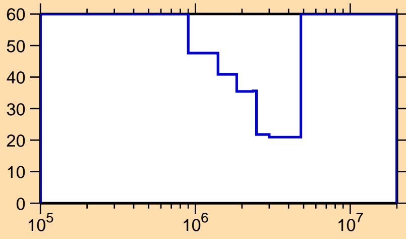
\Delta\sigma/\sigma vs. E for ^{187}\text{Hf}(n,n\text{cont.})
