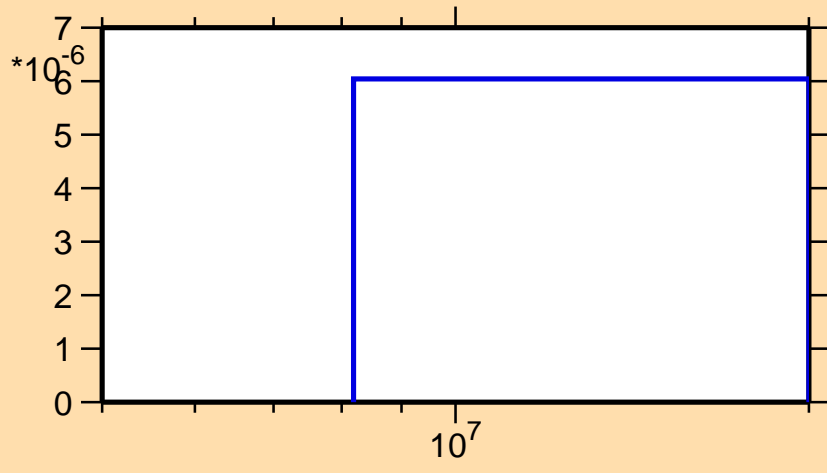
\sigma vs. E for ^{187}\text{Hf}(n,d)
