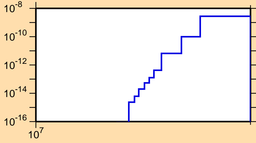
\sigma vs. E for ^{188}\text{Hf}(n,2n\alpha)
