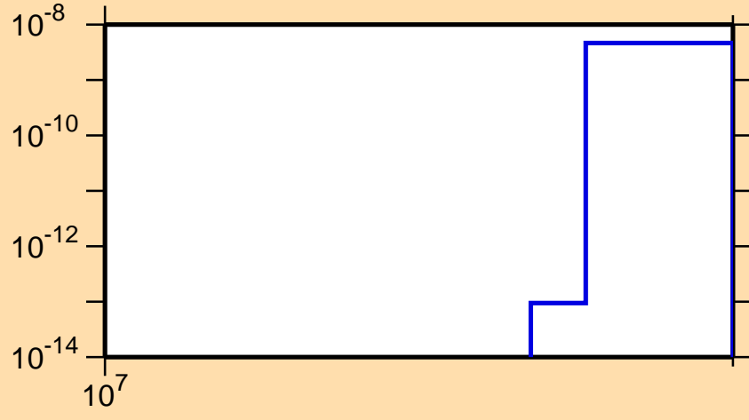
\sigma vs. E for ^{188}\text{Hf}(n,\text{nd})
