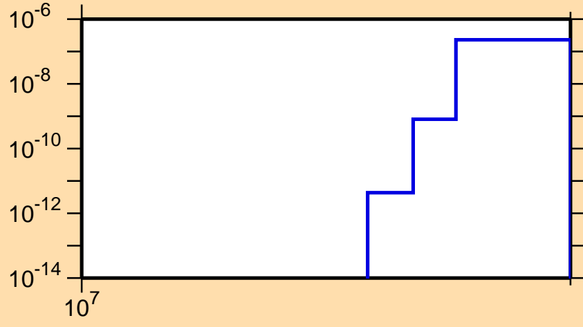
\sigma vs. E for ^{188}\text{Hf}(n,nt)
