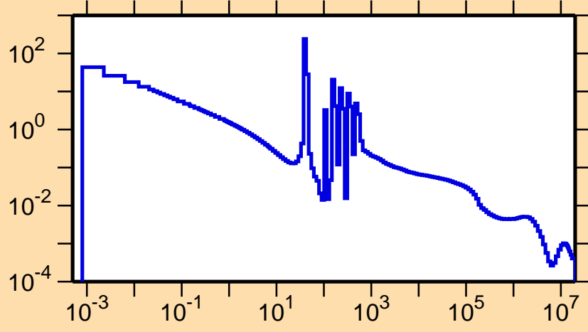
\sigma vs. E for ^{188}\text{Hf}(n,\gamma)
