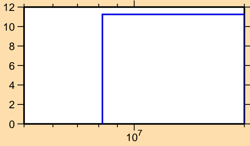
\Delta\sigma/\sigma vs. E for ^{188}\text{Hf}(n,el.)
