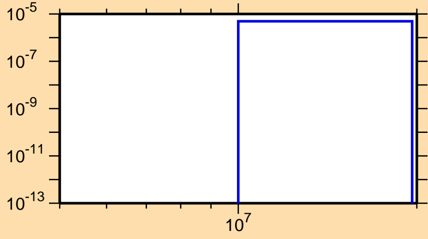
\sigma vs. E for ^{189}\text{Hf}(n,t)
