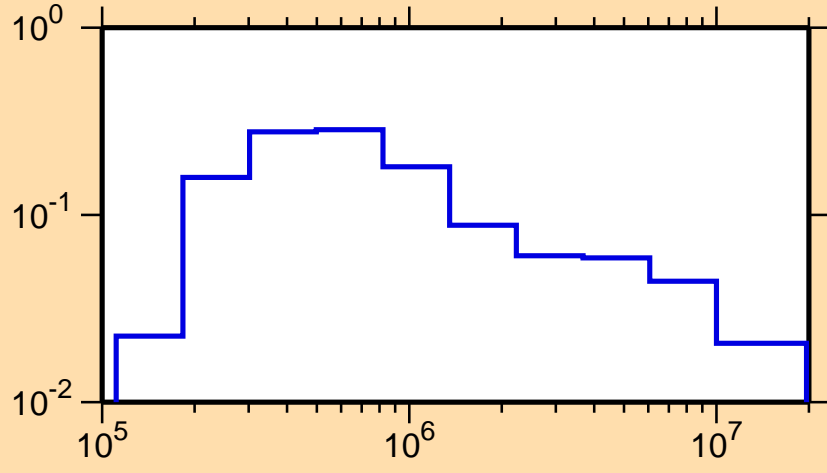
\sigma vs. E for ^{189}\text{Hf}(n,n_1)
