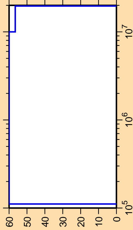
\Delta\sigma/\sigma vs. E for ^{189}\text{Hf}(n,n_1)
