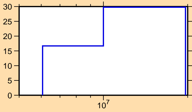
\Delta\sigma/\sigma vs. E for ^{189}\text{Hf}(n,2n)
