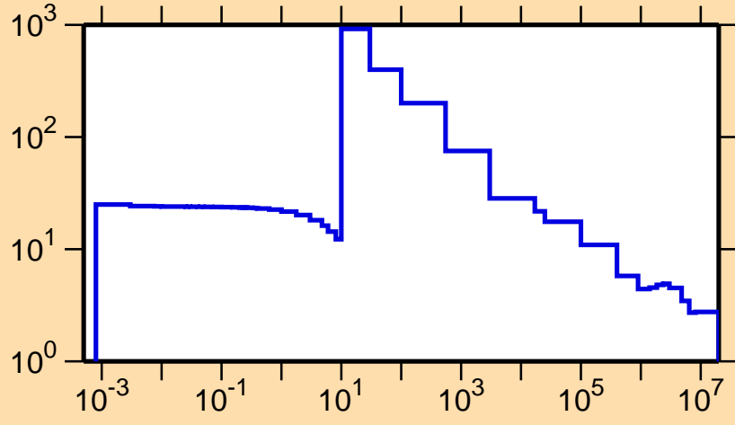
\sigma vs. E for ^{189}\text{Hf}(n,\text{el.})
