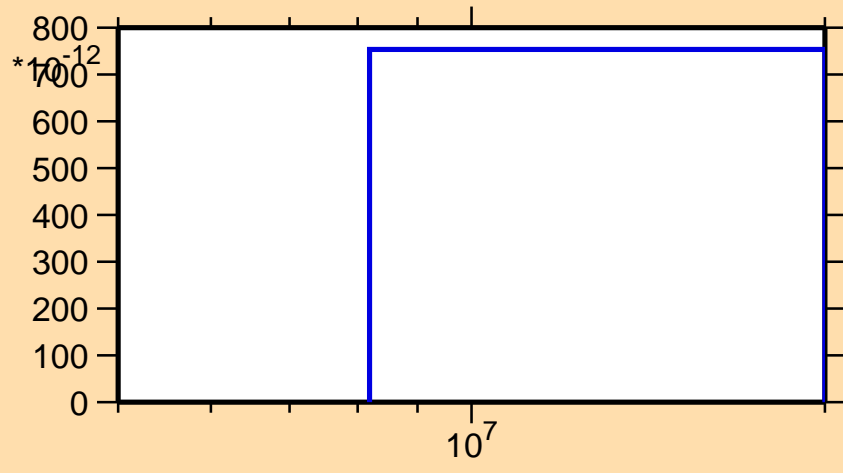
\sigma vs. E for ^{189}\text{Hf}(n,nd)
