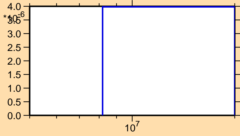
\sigma vs. E for ^{189}\text{Hf}(n,t)
