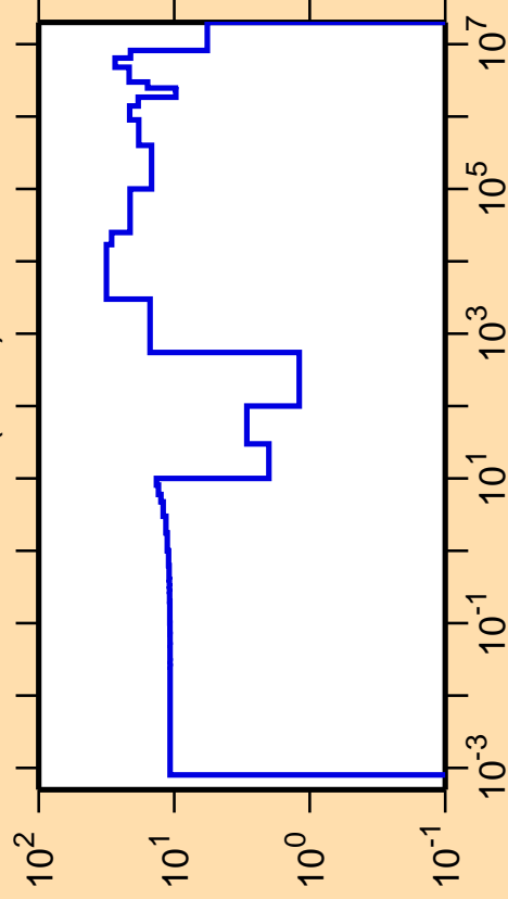
\Delta\sigma/\sigma vs. E for ^{189}\text{Hf}(n,\text{el.})
