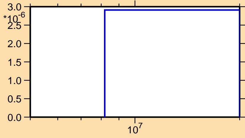
\sigma vs. E for ^{189}\text{Hf}(n,d)
