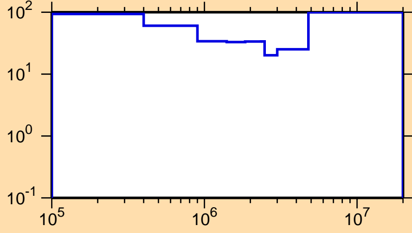
\Delta\sigma/\sigma vs. E for ^{189}\text{Hf}(n,n\text{cont.})
